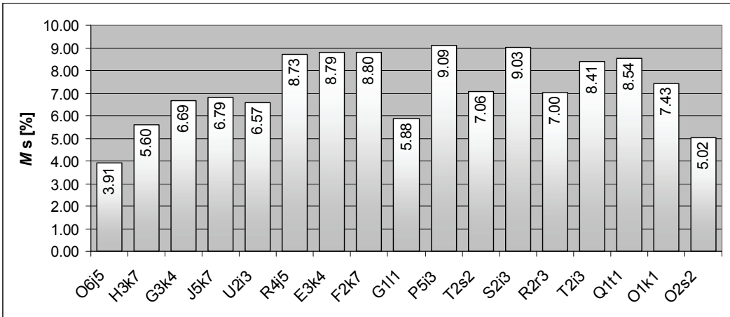
Fig. 14. Averaged value of the mismatch of simulated laser parameters for different lasers: M_s is for electron density characteristic (Vasiliauskas et al., 2007)
