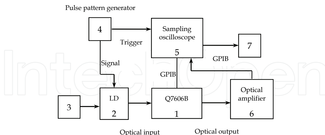
Fig. 2. Chirp measurement setup. (1) Mach-Zehnder fiber interferometer (Advantest Q7606B Optical Chirpform Test Set), (2) semiconductor laser, (3) direct current source (ILX Lightwave LDC-3900 modular laser diode controller), (4) pulse pattern generator (Agilent HP-70843B error performance analyzer), (5) signal analyzer – digital sampling oscilloscope (Tektronix TDS8000 Digital Sampling Oscilloscope), (6) erbium doped fiber amplifier, (7) personal computer with integrated General Purpose Interface Bus (GPIB) interface
