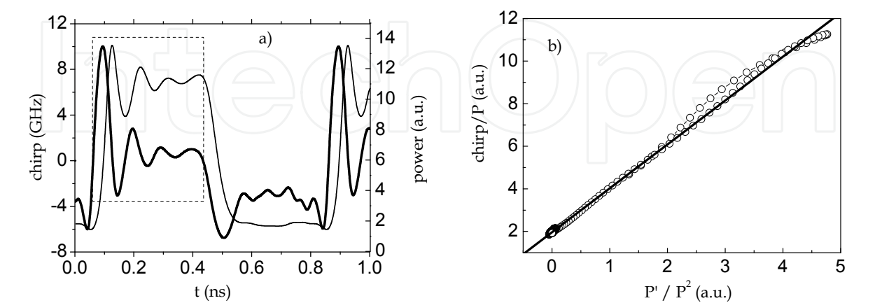
Fig. 8. Chirp parameter extraction in case of a 2.5 Gbit/s modulation rate. Frequency chirp and optical beam power waveform a), linearised time-resolved frequency chirp waveform b) (Šermukšnis et al., 2005)
