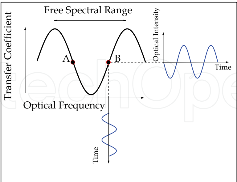
Fig. 3. Mach-Zehnder interferometer frequency transfer function
