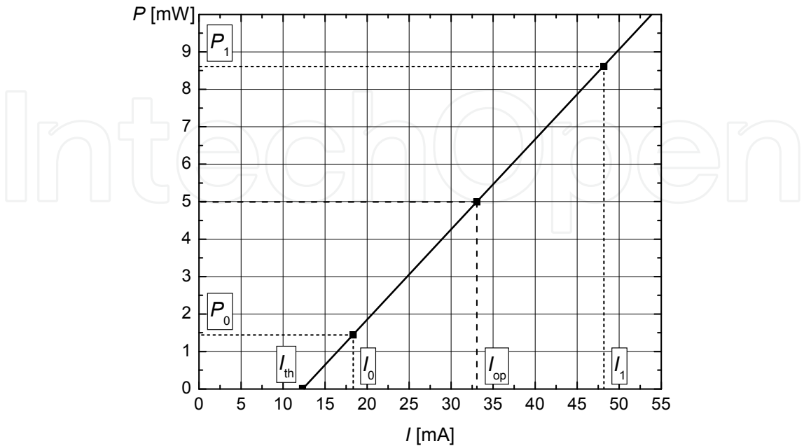
Fig. 11. Optical power dependence on injection current (Vasiliauskas et al., 2007)
