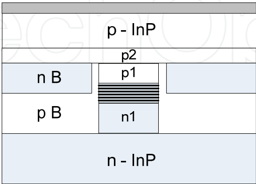
Fig. 1. Schematic diagram of the finished laser structure in the vicinity of the mesa. p-InP p:10 18 cm -3 , p2-InP p:10 18 cm -3 , p1-InP p:5·10 17 cm -3 , n1-InP n:10 18 cm -3 , n -InP n:10 18 cm -3 nB-InP n:10 18 cm -3 , pB-InP p:6·10 17 cm -3 . Active region of the InGaAsP MQWs is formed between p1 and n1 layers.
