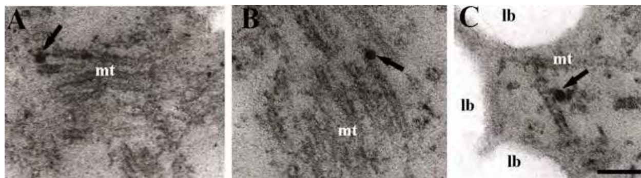
Fig. 18. O. umbellatum microtubules in longitudinal sections (A-C) with 20 nm gold grains at the surface indicating the presence of phospholipase D (arrows); lb – lipid bodies, mt – microtubules; bar: 100 nm (Kwiatkowska et al., 2011b).
