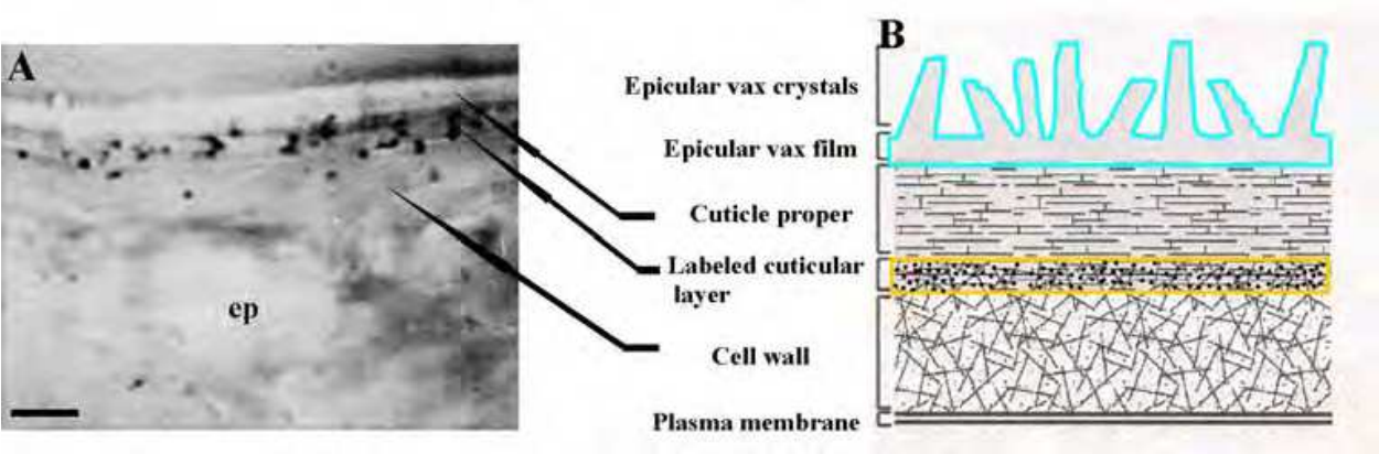
Fig. 21. A - Cross-section of O. umbellatum ovary epidermis (ep); autoradiogram after 2 h incubation in 3 H-palmitic acid, 6 h postincubation in the non-radioactive medium and after extraction in the lipid solvent; silver grains localized in the cuticular layer (Kwiatkowska et al., in prep.); B - a scheme of cuticle according to Bird (2008 - modified); bar: 5 μm.
