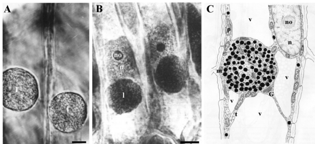
Fig. 1. Ornithogalum umbellatum “elaioplast” (lipotubuloid); A – in a living cell; B – after \text{OsO}_4 fixation; C – a scheme of epidermis cell with lipotubuloid; G – Golgi apparatus, l – lipotubuloid, lb – lipid bodies, m – mitochondrion, n – nucleus, no – nucleolus, p – plastid, t – tonoplast, v – vacuole; bars: 10 \mu\text{m} .
