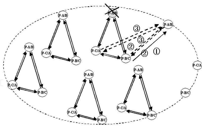
Fig. 3. P-Node (A/B) replacement process
