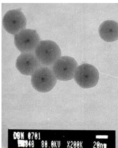
Fig. 9. TEM image of ZnS:Mn@silica nanoparticles with a core – shell structure. (Reproduced with permission, Dong B. et al. 2009).
