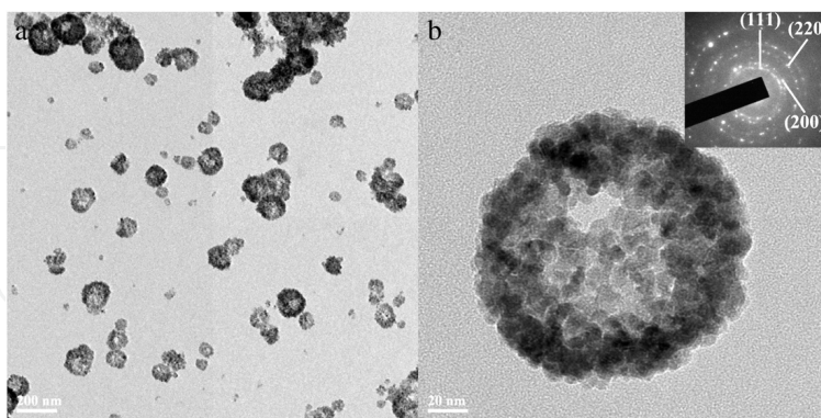
Fig. 10. TEM image of the Ni hollow spheres and (b) a single Ni hollow sphere. Inset: SAED pattern. Reproduced with permission (Jiang et al., 2010).
