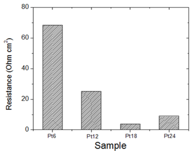
Fig. 5. Bulk resistance of Pt catalysts prepared by potential sweep method as a function of sweep times.
