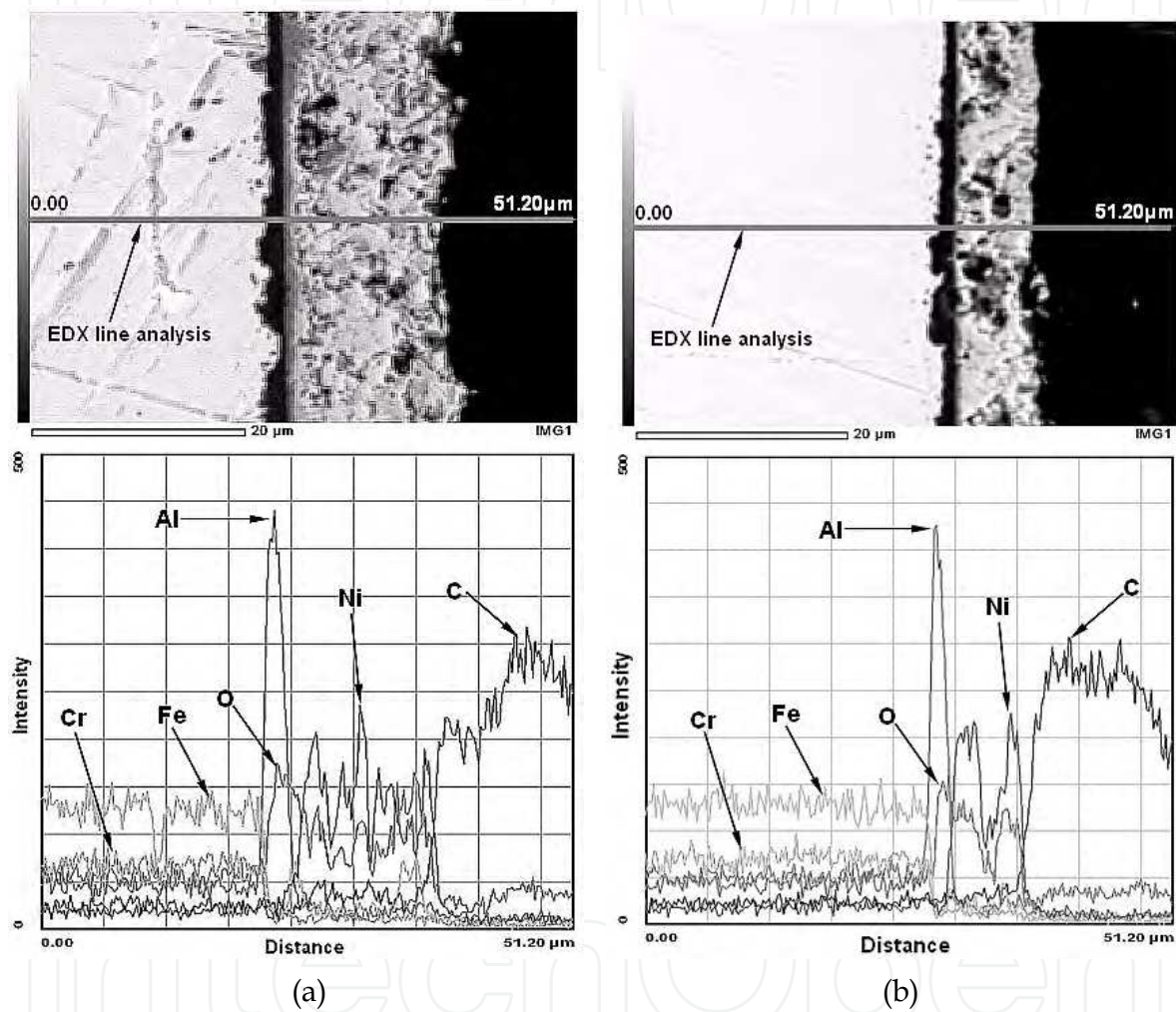
Fig. 17. Cross section scanning electron micrograph showing EDX line analysis (from left to the right) of FeCrAl ultrasonic with (a) SiC for 50 minutes, (b) Al 2 O 3 for 30 minutes prior to nickel electroplating and oxidized at 900 °C with its chemical's intensity graph
