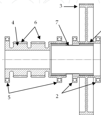
Fig. 12. Conventional assembly of a quill shaft
