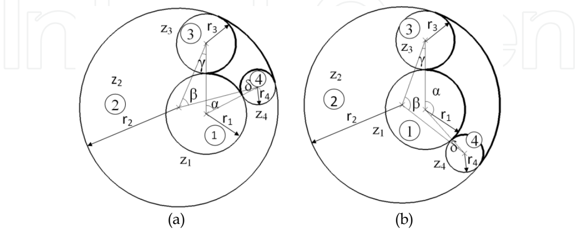
Fig. 8. Solutions for three outside gears and one ring gear: (a) crossed quadrilateral (b) non-crossed quadrilateral
