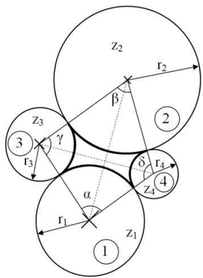
Fig. 6. Nomenclature for the four-gear case
