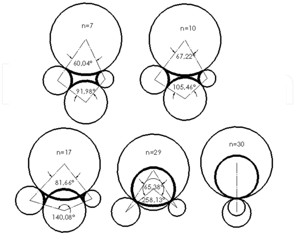
Fig. 7. Feasible solutions for given numbers of teeth
