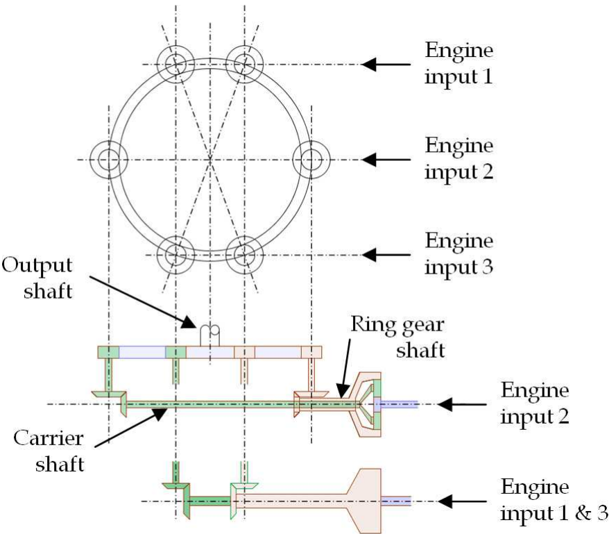
Fig. 10. Schematic view of split torque main transmission
