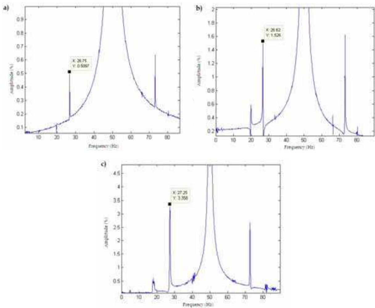
Fig. 16. a) Healthy motor; b) e=44.5%; c) e=87.3%
