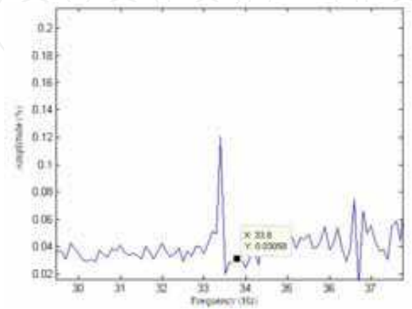
Fig. 24. Short-circuit associated frequency
