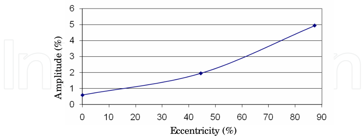
Fig. 17. Failure amplitude vs. eccentricity
