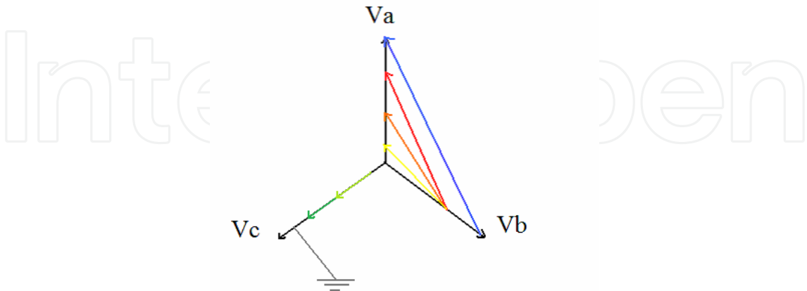
Fig. 7. Different types of short-circuit. In blue, orange, yellow and red the short-circuits are between two phases of different magnitudes. In gray a ground fault is represented and in green two shorts of the same phase of different magnitudes (these defects are the ones that will be simulated)
