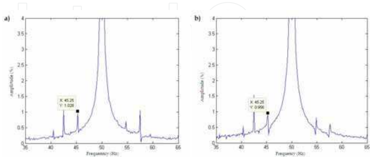
Fig. 6. a) One broken bar; b) Five broken bars
