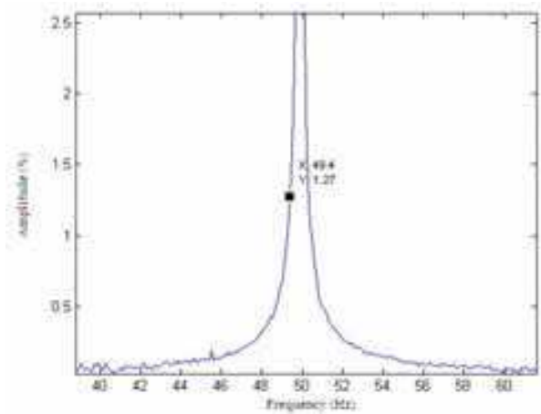
Fig. 23. Broken bars associated frequency
