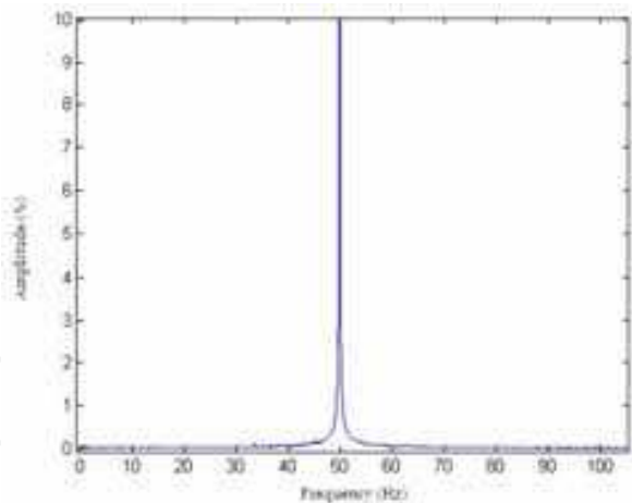
Fig. 21. Normalized FFT of the sampled signal
