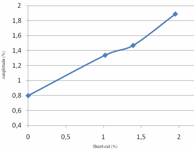
Fig. 10. Amplitude vs. short-cut magnitude
