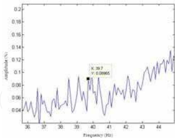
Fig. 25. Bearing damage associated frequency
