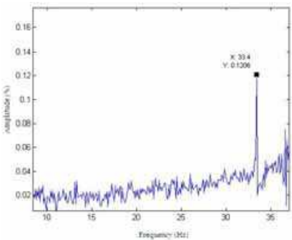
Fig. 26. Eccentricity associated frequency
