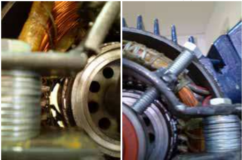
Fig. 18. Eccentricity failure
