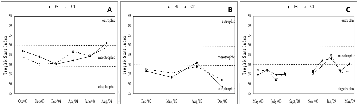
Fig. 4. Seasonal variation of Trophic State Index (TSI) for FS and CT for Nova Avanhandava (A), Jurumirim (B) and Chavantes (C) reservoirs.
