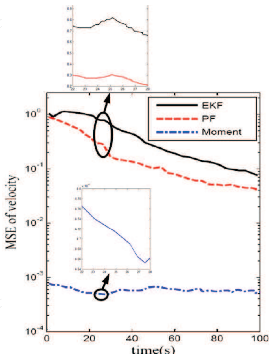
Fig. 8. MSE of estimated velocity in the conventional and proposed methods for SNR=+10 dB.
