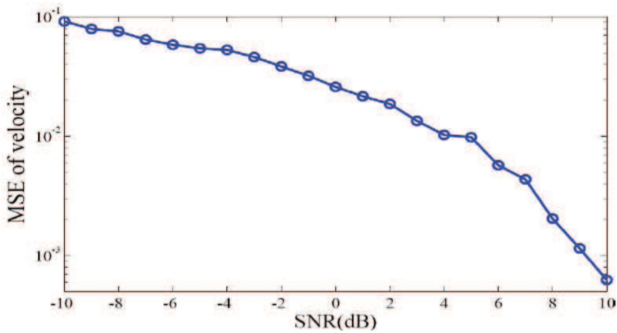
Fig. 10. MSE of estimated velocity in the proposed method.
