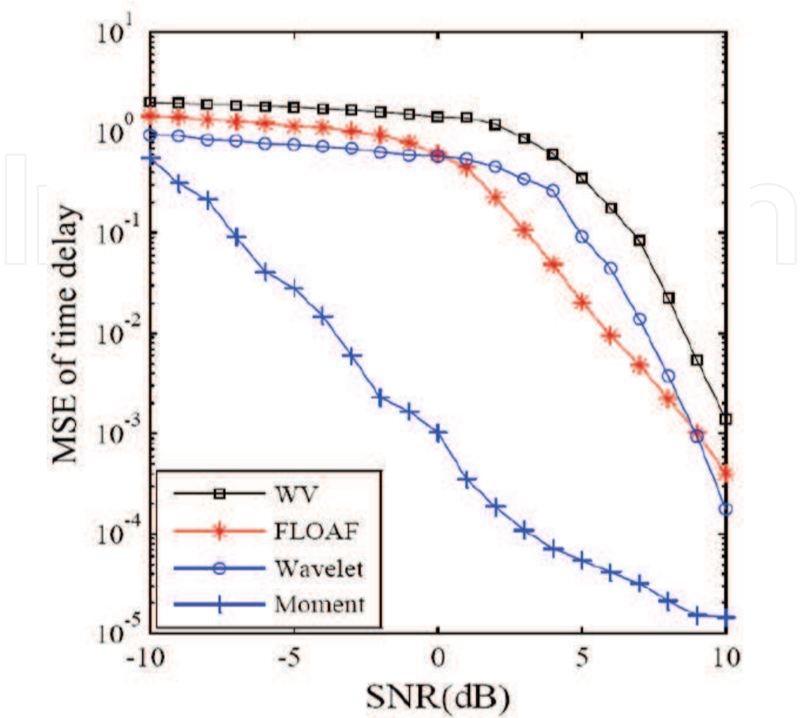
Fig. 4. MSE of estimated time delay in the conventional and proposed methods.
