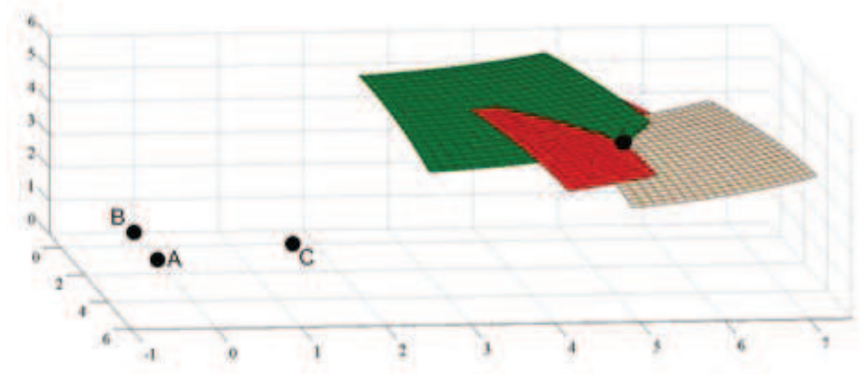
Fig. 3. The position of the three sensors and the intersection of three spheres related to the sensors
