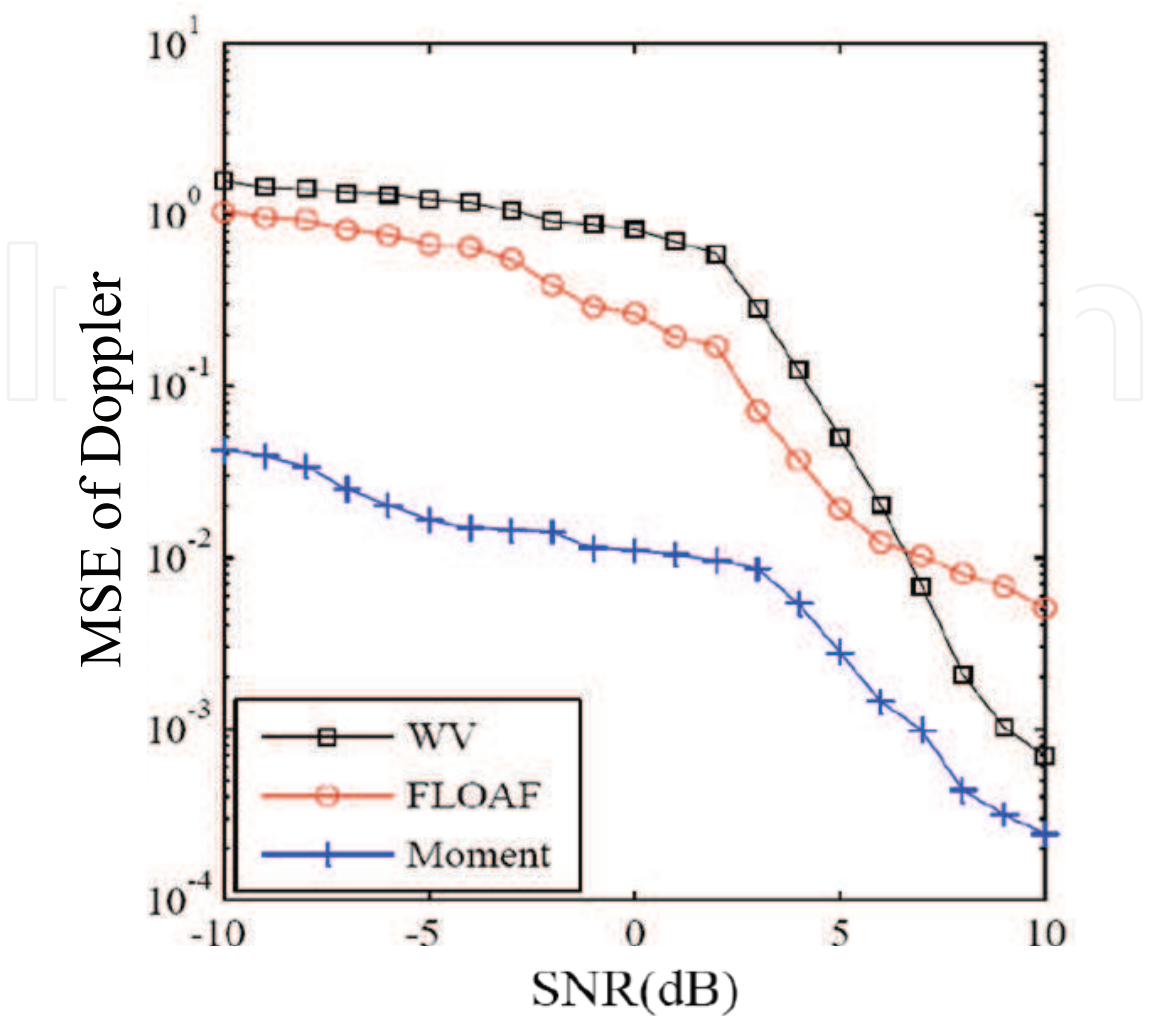
Fig. 5. MSE of estimated Doppler in the conventional and proposed methods.
