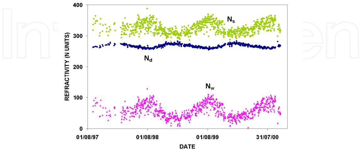
Fig. 3. Evolution of surface refractivity ( N_s ) and the wet ( N_w ) and dry terms ( N_d ) over Barcelona (Bech, 2003).
