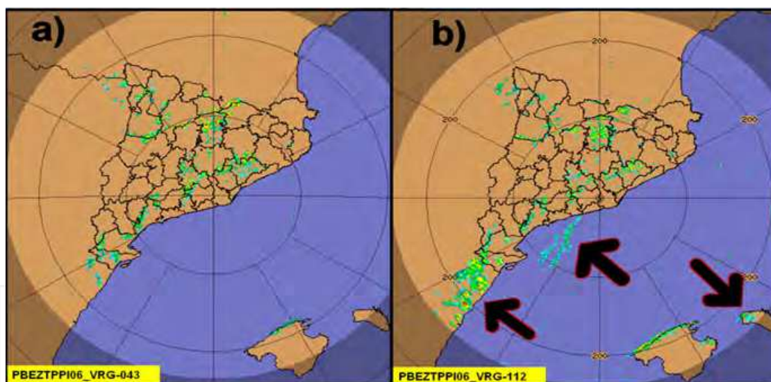
Fig. 2. Radar reflectivity base PPI images ( 0.6^{\circ} ) with no Doppler filtering showing ground and sea clutter on a normal propagation day (a) and a superrefractive day (b). Arrows indicate new or more intense AP echoes.
