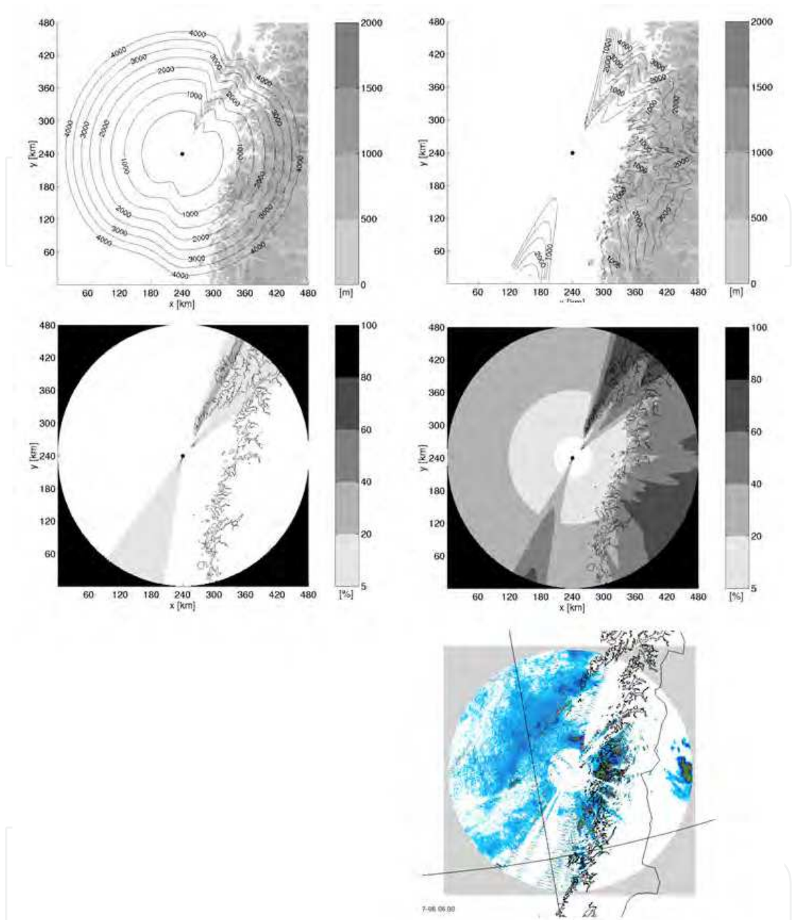
Fig. 16. Lowest unblocked radar coverage (top row) and beam blockage (middle) computed with radiosonde data (left column) and NWP-derived profiles (right column). The bottom panel shows actual radar observations, 6 July 2005 00 UTC (Røst radar, met.no). Adapted from Bech et al. (2007a).
