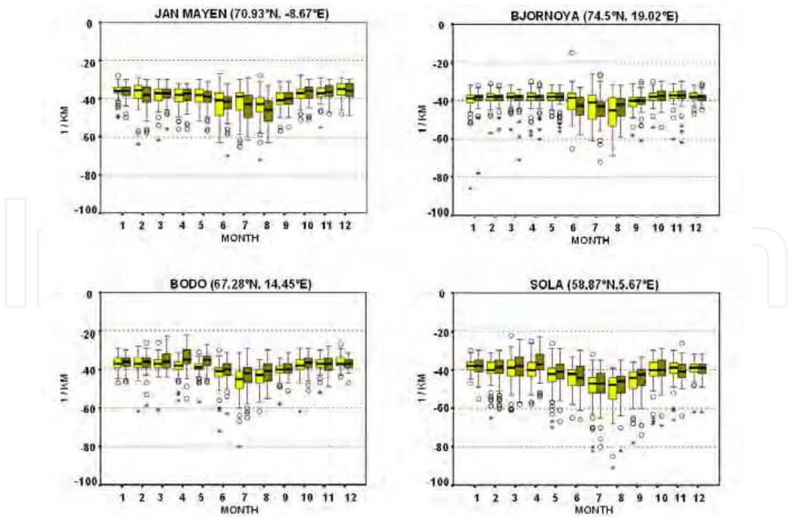
Fig. 6. Box-whisker plots for several Norwegian radiosonde sites showing 00 Z (clear boxes) and 12 Z (dark boxes) data. Adapted from Bech et al. (2007b).
