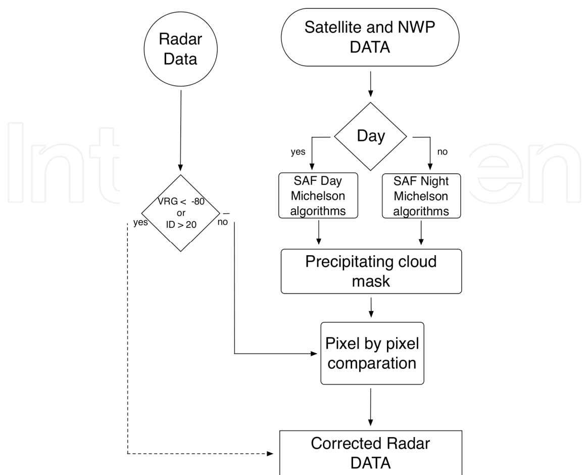
Fig. 18. Flow diagram showing the main processes involved in the algorithm to detect radar AP echoes with precipitating cloud masks derived from satellite images. Adapted from Magaldi et al. (2009).
