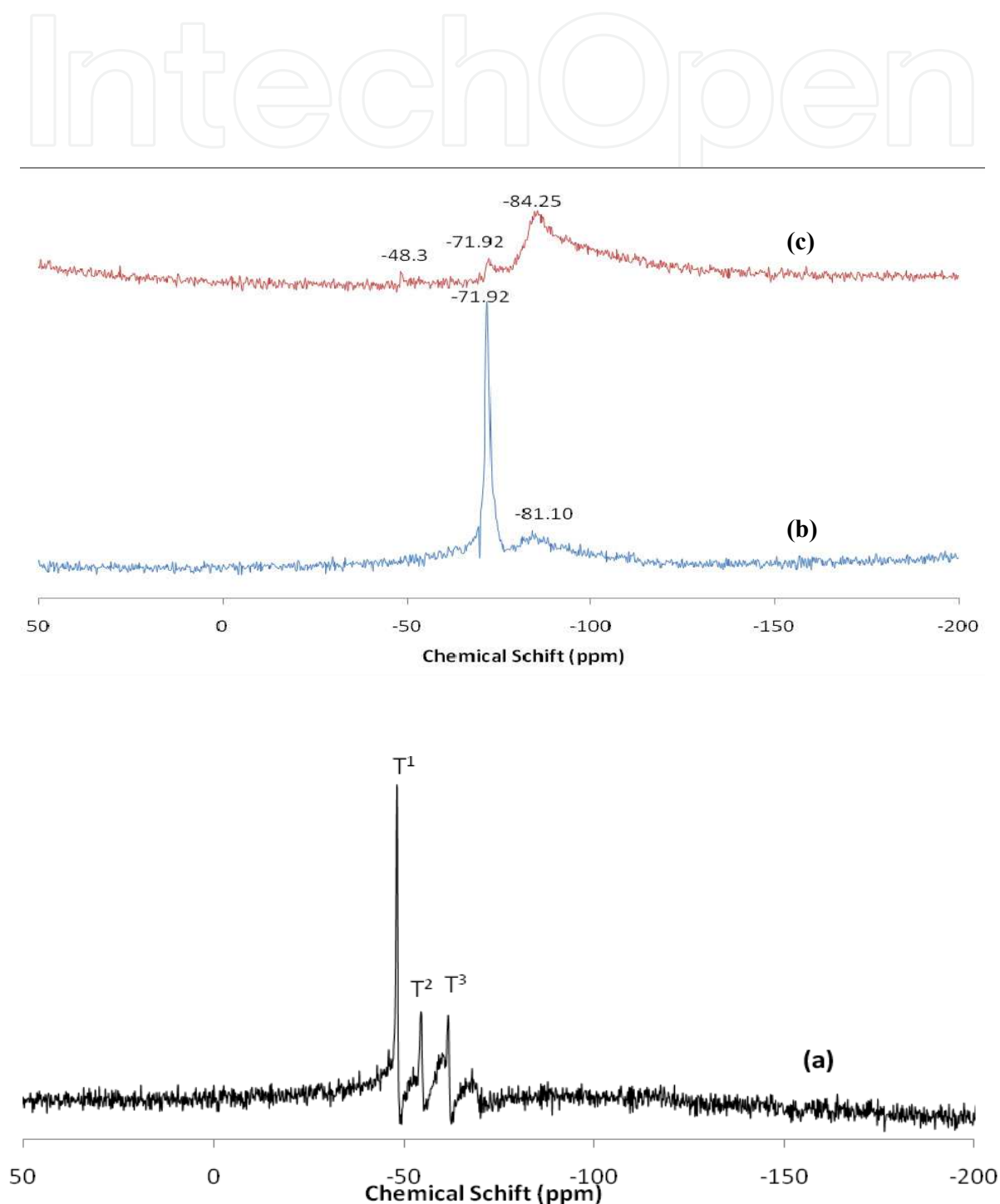
Fig. 16. ^{29}\text{Si} CP-MAS NMR spectra of: (a) Fluoroalkylsilane molecule (b) ungrafted membrane, (c) microfiltration grafted membrane.
