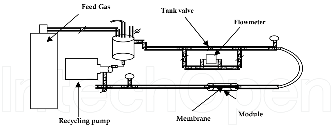
Fig. 10. Flow schema of experimental apparatus.
