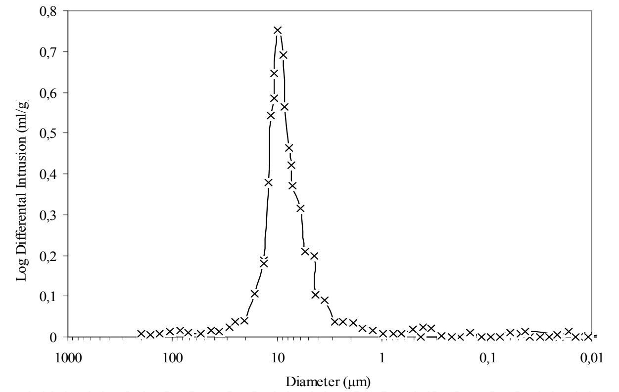
Fig. 5. Pore diameters of the silty marls supports.
