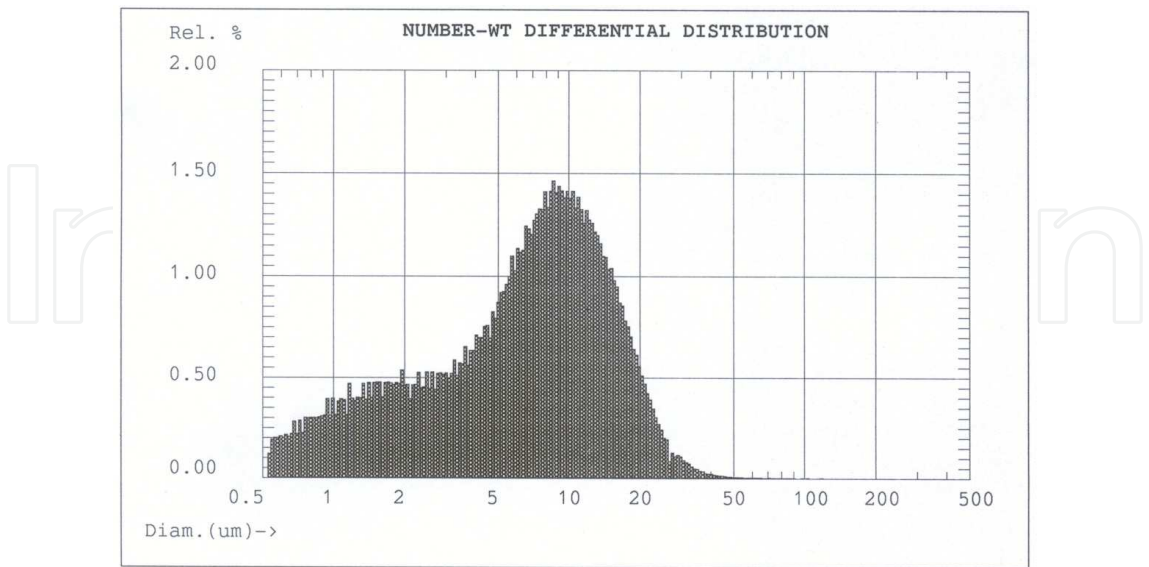
Fig. 2. Silty marls (M11) particle size distribution.
