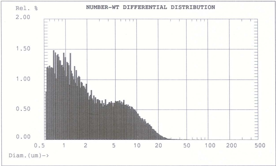
Fig. 6. Clay (JM18) particle size distribution.
