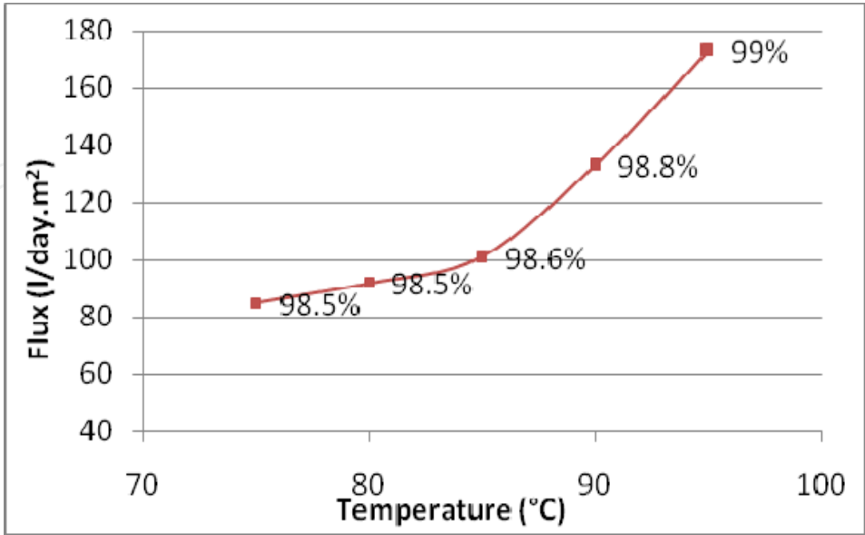
Fig. 19. Variation of the permeate flux as a function of the temperature. The values reported on the graph correspond to the rejection rates calculated for the different membranes after filtration of seawater.
