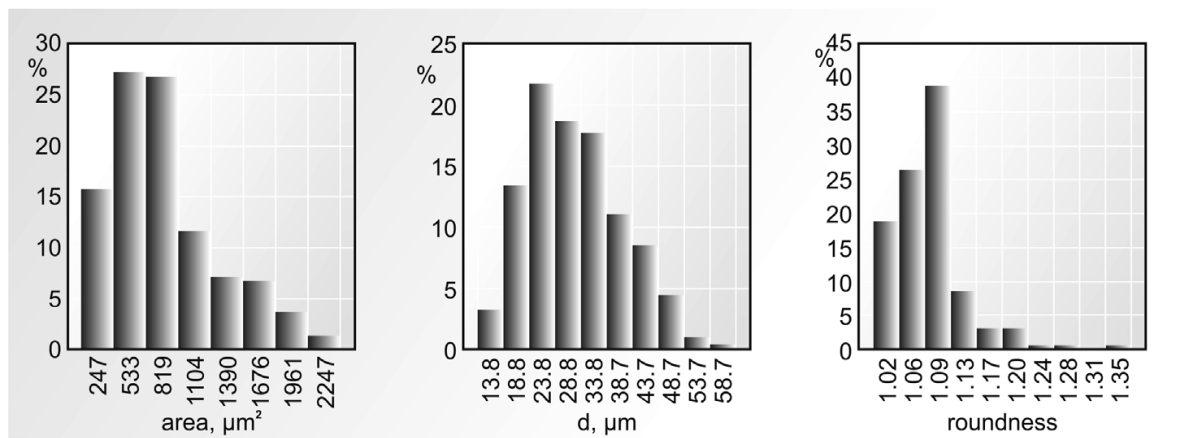
Fig. 16. Surface area histogram in particle of \text{ZrO}_2 + 20\text{wt.}\% \text{Y}_2\text{O}_3 powder Fig. 17. Chord histogram in particles of \text{ZrO}_2 + 20\text{wt.}\% \text{Y}_2\text{O}_3 powder Fig. 18. Shape factor histogram in particles of \text{ZrO}_2 + 20\text{wt.}\% \text{Y}_2\text{O}_3 powder
