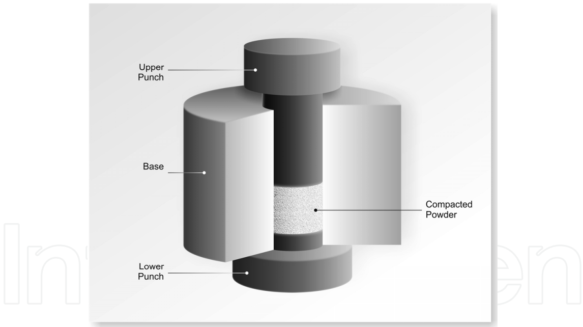
Fig. 19. Diagram of the mould used for powder compaction
