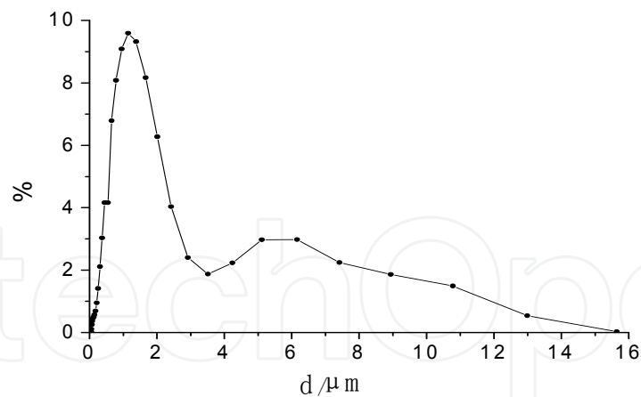
Fig. 1. Particle size distributions of TiB 2 powder
