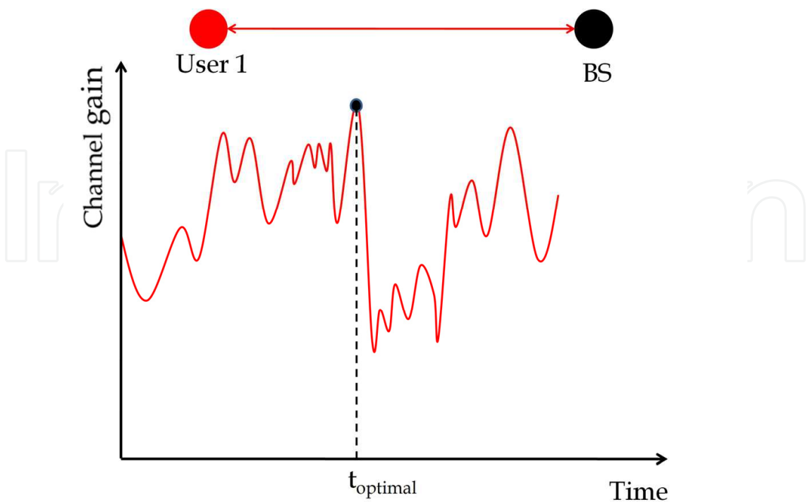
Fig. 2. Time diversity
