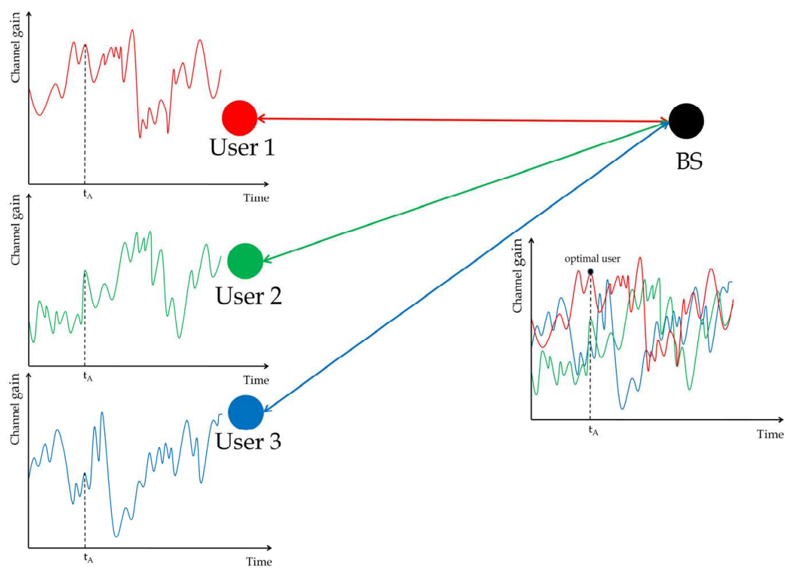
Fig. 3. Multi-user diversity
