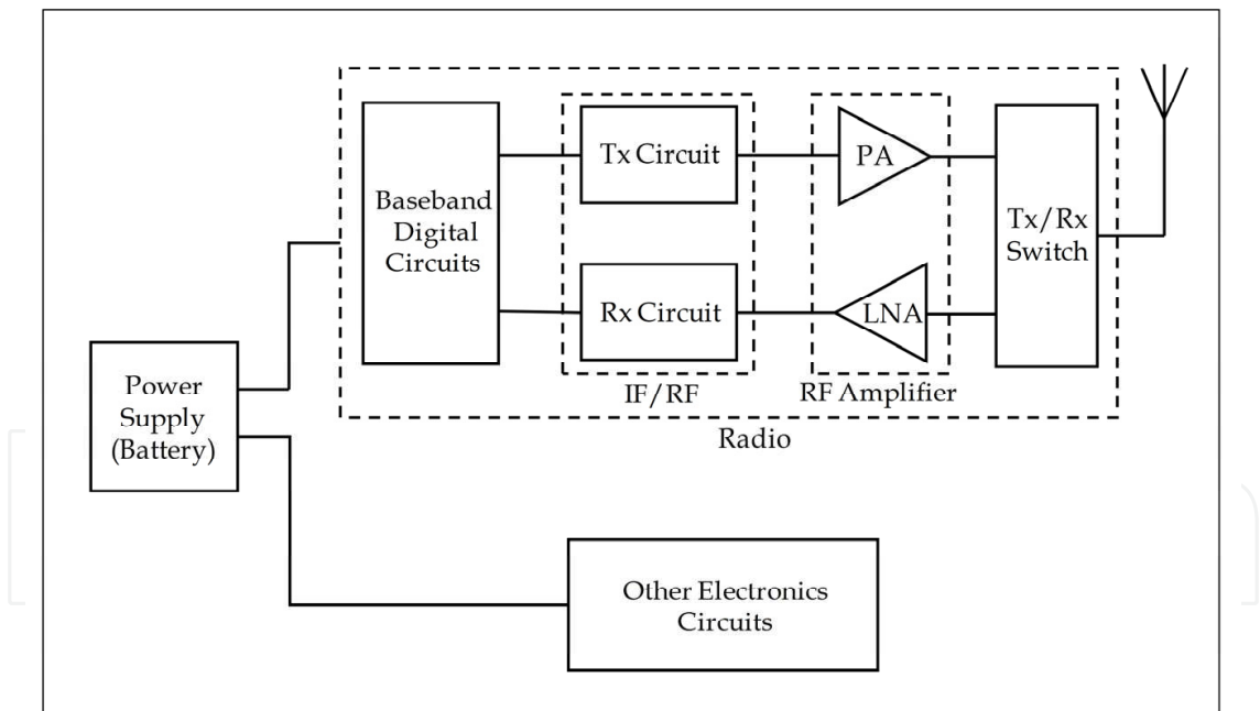
Fig. 1. A simple structure of wireless communication module
