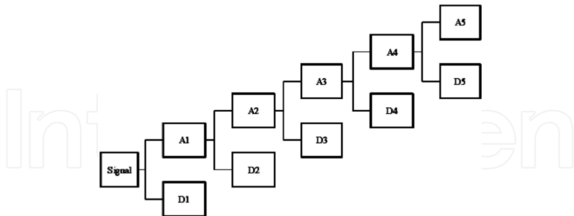
Fig. 2. Decomposition tree for DWT
