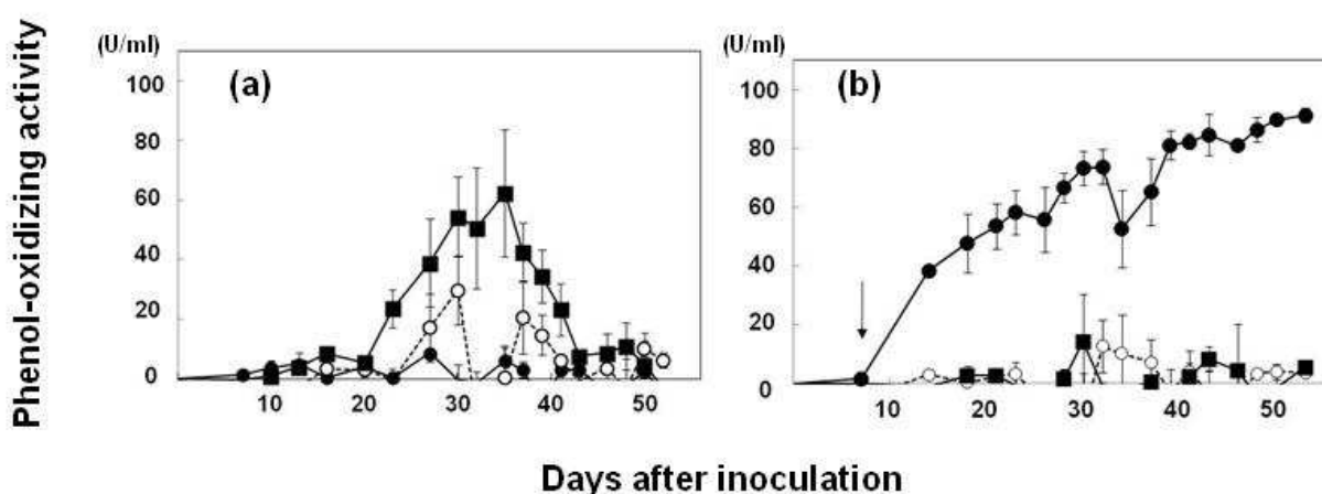
Fig. 3. Changes of phenol-oxidizing activities of (●) Lcc, (○) Per and (■) MnP in a liquid culture medium of L. edodes under (a) MnP-induced (MYPG-S) or (b) Lcc-induced conditions (MYPG-S with 2mM \text{CuSO}_4 \cdot 5\text{H}_2\text{O} ) (reprinted from Saeki et al., 2011). The arrow in panel (b) indicates the day of 2 mM \text{CuSO}_4 \cdot 5\text{H}_2\text{O} addition. Values are means with standard errors (vertical bars) for three replicate cultures.
