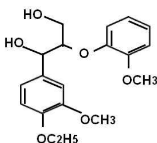
Fig. 2. \beta -O-4 lignin model compound used in this study; 4-ethoxy-3-methoxyphenylglycerol- \beta -guaiacyl ether (from Umezawa & Higuchi, 1985).
