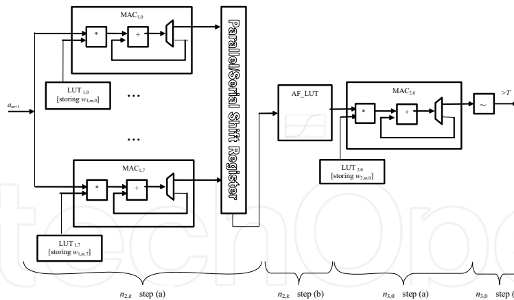
Figure 15. PCAC functionality
