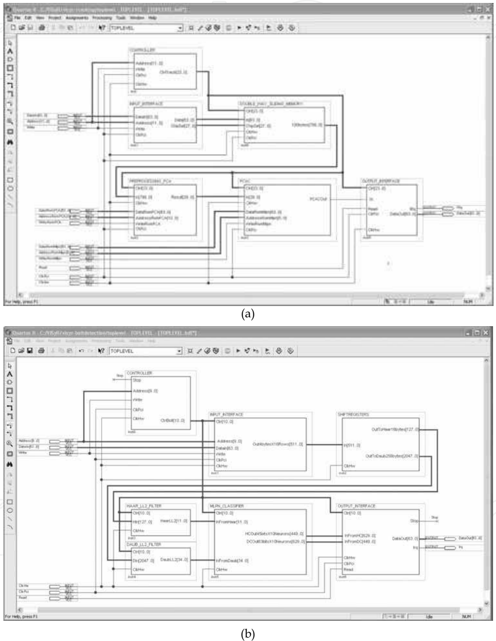
Figure 13. A top-level schematic of (a) RD&TB and (b) BDB, as they can be displayed on Altera’s QuartusII™ CAD tool
