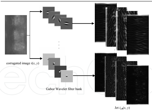
Figure 12. Example of Gabor Wavelet transform of the corrugated image We have applied the GWT, combining the parameters applied to the Gabor Filter case and to the DWT case, i.e., applying three decomposition levels and four orientations ( 0, \pi/2, 3/4
