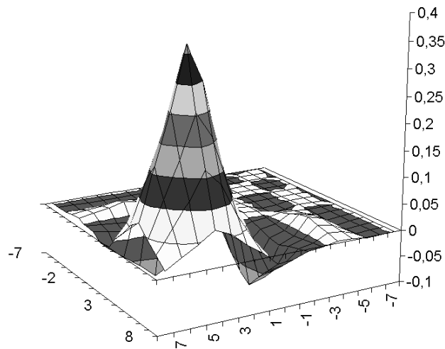
Figure 16. Symmetrical 16 \times 16 kernel for directly computing in one 2-D step the LL_2 subband of the DWT based on the 1-D low-pass filter. The filtering has to be followed by decimation by 4 along both rows and columns
