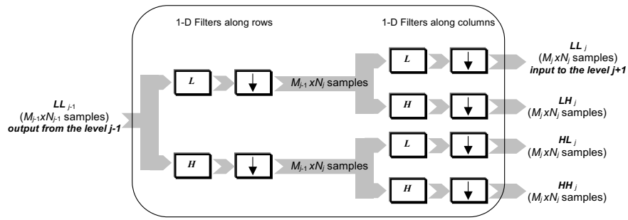
Figure 23. 2-D DWT: The j^{th} level of subband decomposition. \downarrow represents decimation by 2
