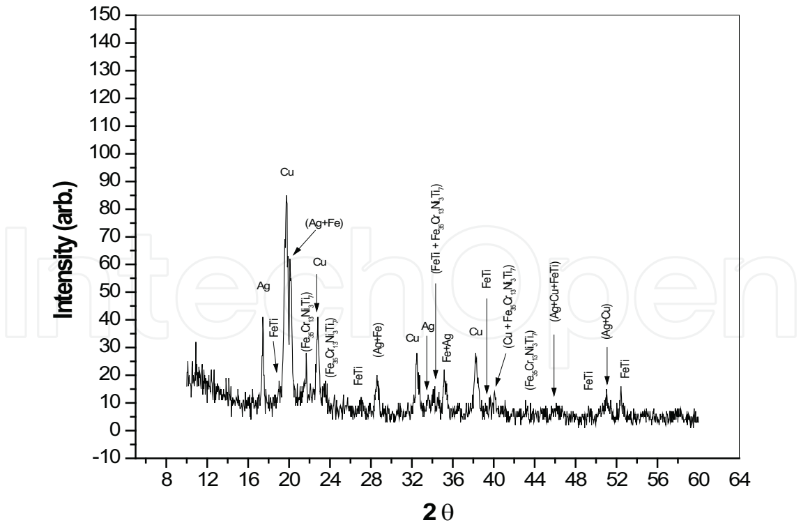
Fig. 4. (b) X-ray diffraction patterns (XRD) of Al 2 O 3 - SS brazed joint: pattern '5' of the above figure adjacent to SS interface. MoK α radiation, Figure identifies the presence of FeTi and Fe 35 Cr 13 Ni 3 Ti 7
