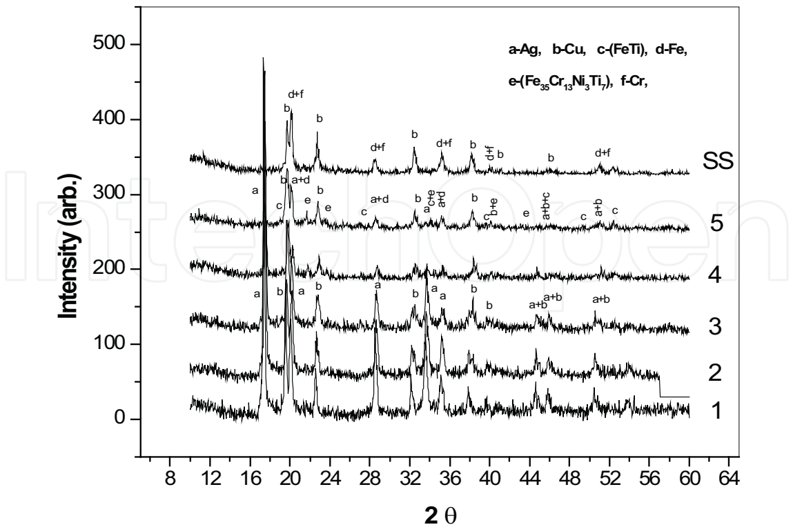
Fig. 4. (a) X-Ray diffraction patterns (XRD) of Al 2 O 3 -304 SS brazed joint. Some of the most relevant diffraction patterns taken from the SS interface are depicted. MoK α radiation
