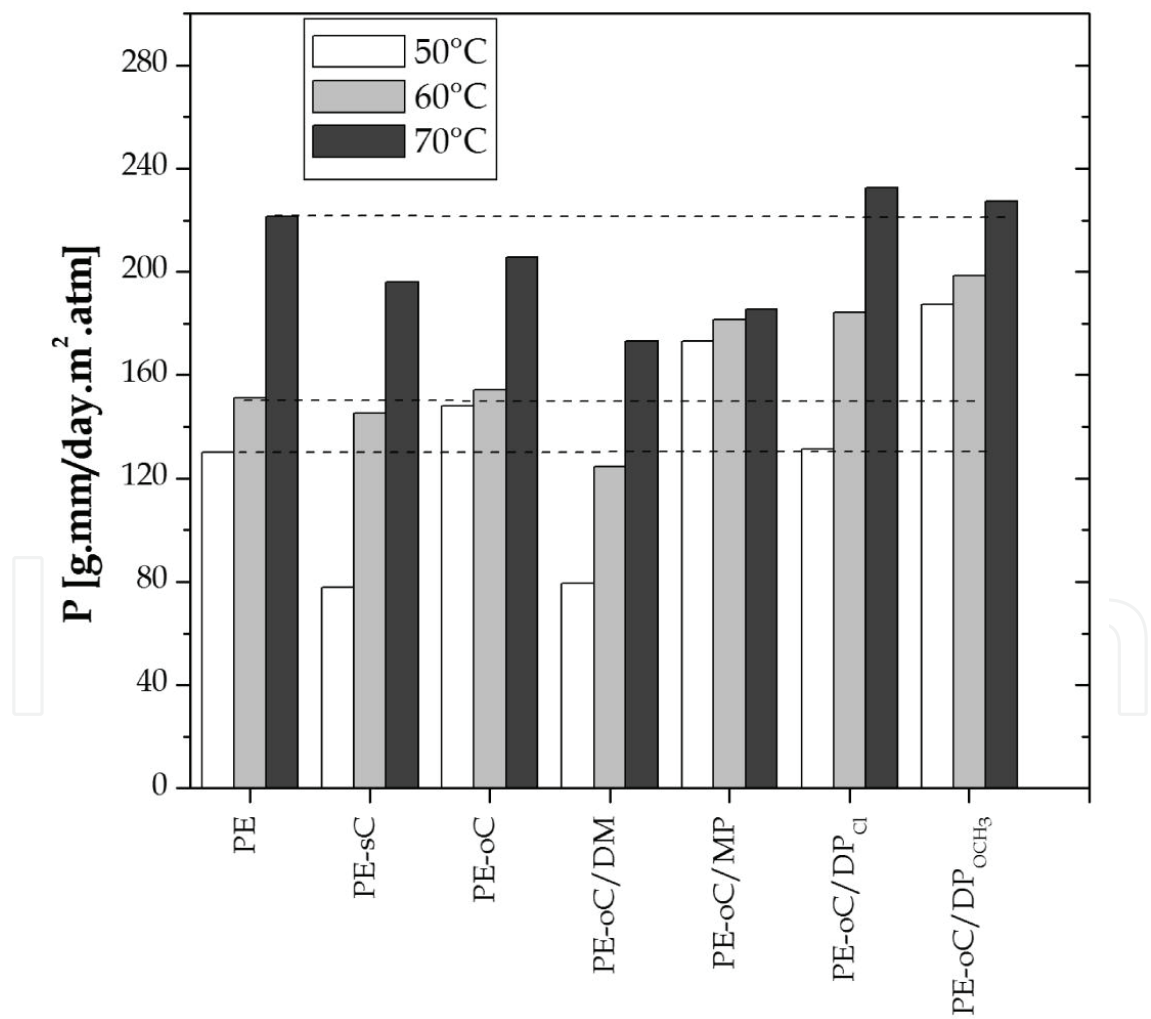
Fig. 10. Permeability coefficients of the prepared composites, compared to PE polymer (Monasterio & Destéfanis, 2011).
