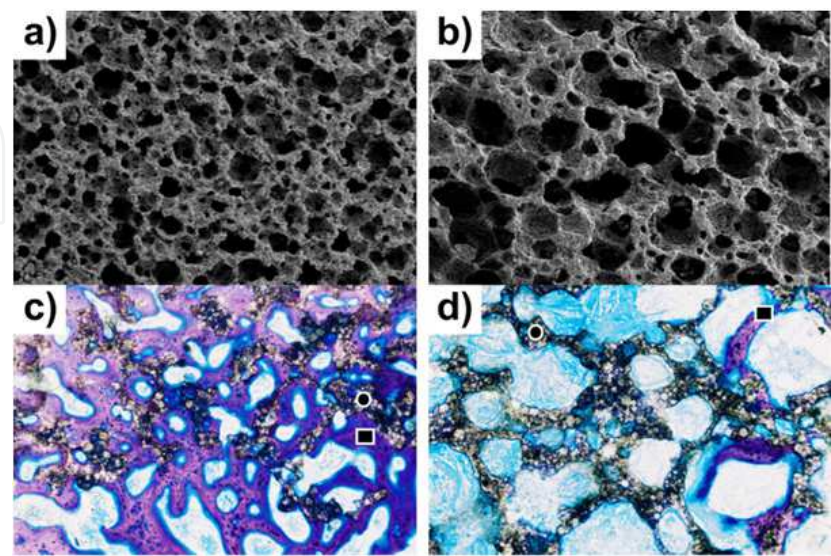
Fig. 10. SEM images of TCP-Ss and T.B staining of femur of beagle at after 3 weeks implanted. a), c): TCP(AN) b),d): TCP(NI) a), b):SEM image c), d): T.B. staining(Enlarged image of Fig.9-c and 9-f) ○ : TCP-S □: New bone The AN specimen showed better early bone formation, and in an extended image, some parts of the TCP-S particles were closely surrounded by newly formed bone. On the other hand, the NI specimen showed that there was a gap between the material and new bone tissue.
