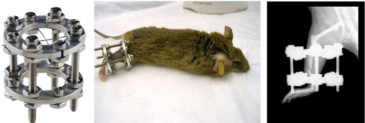
Fig. 10. Mini Ilizarov circular frame applied to a mouse model of DO in our laboratory , and developed by Tay et al. (Tay et al., 1998).
