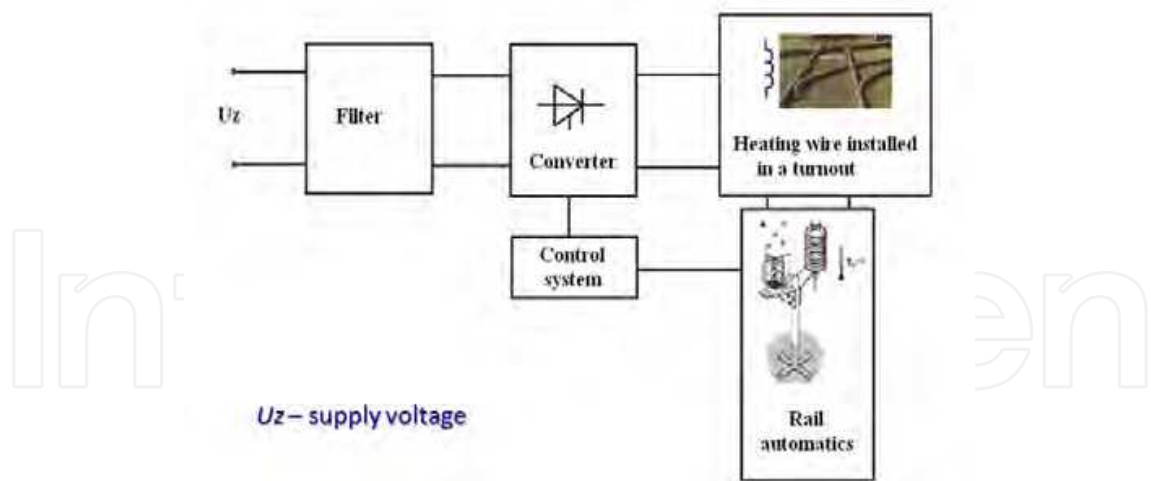
Fig. 6. System of induction turnout heating
