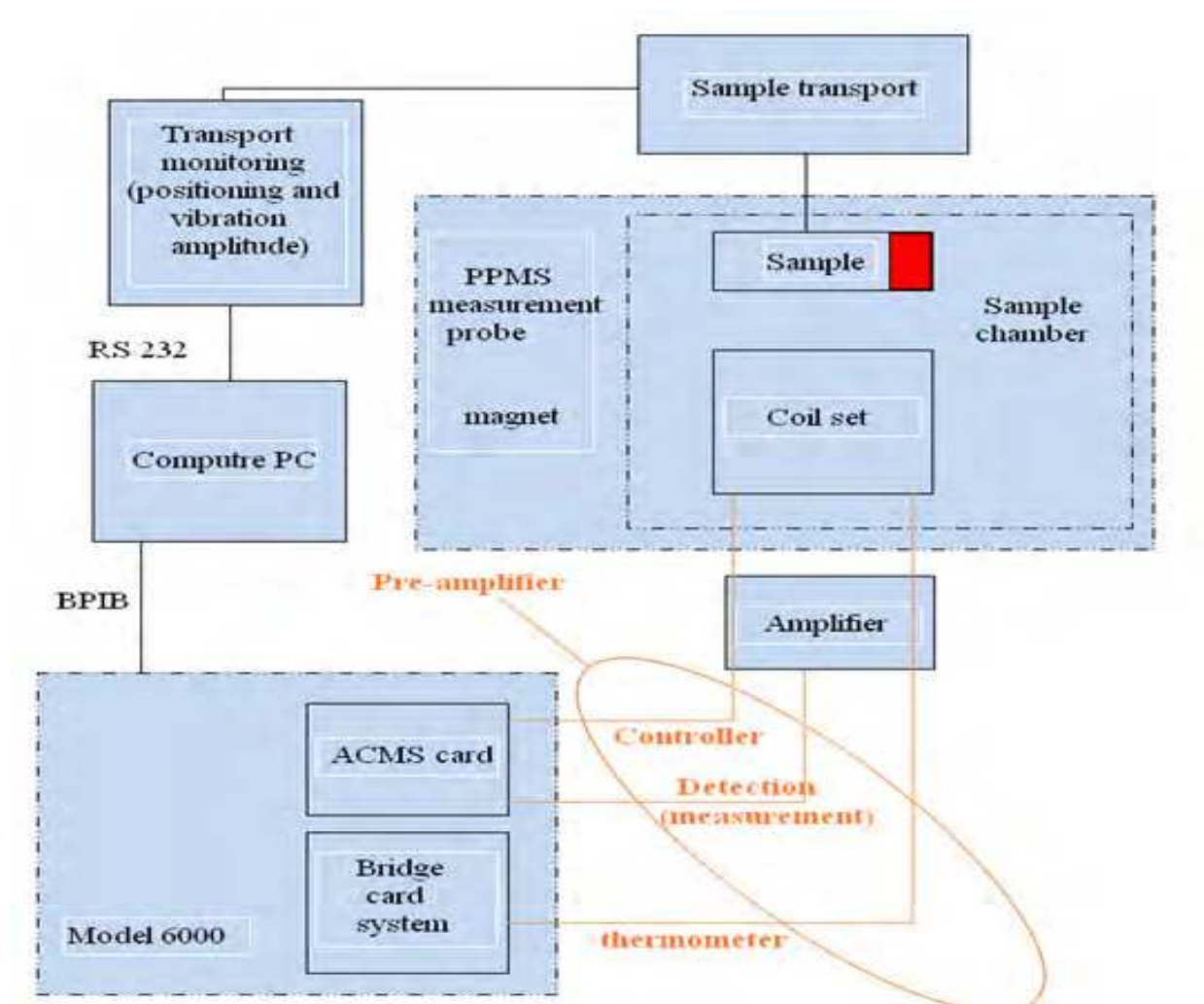
Fig. 18. Flow diagram of ACMS
