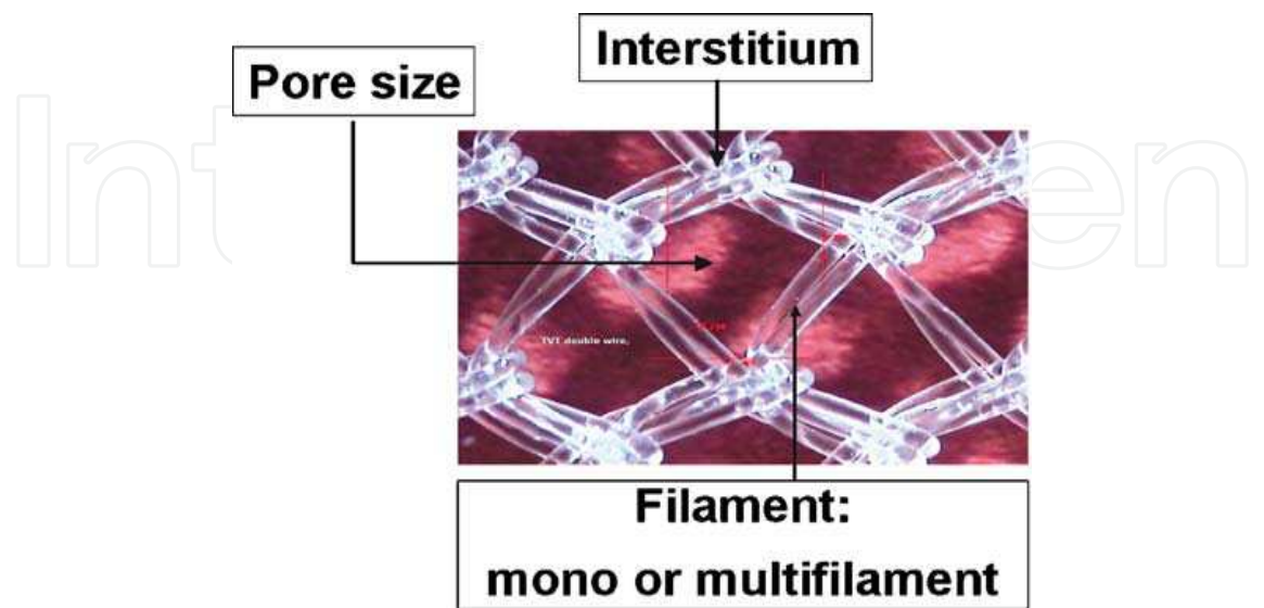
Fig. 3. Terminology used to classify synthetic implants. Magnified view of a part of a polypropylene tape as used for TVT procedure (Gynaecare, Johnson and Johnson) with identification of filament type, interstitium, and pore size (Deprest et al, 2006).
