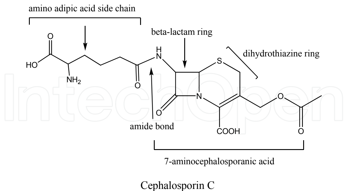
Fig. 1. The structure of Cephalosporin
