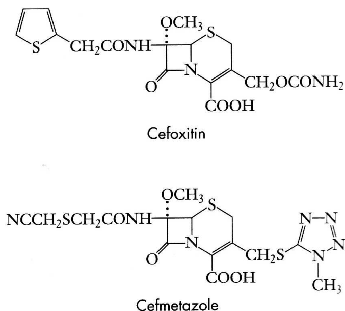
Fig. 6. Second generation Cephalosporins
