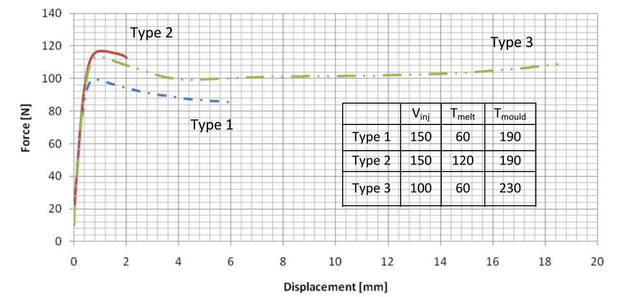
Fig. 7. Force vs displacement curves of three samples: type 1-ductile tensile behaviour with local striction, type 2-brittle behaviour with small deformation at break and type 3-very ductile with long striction and hardening strain.
