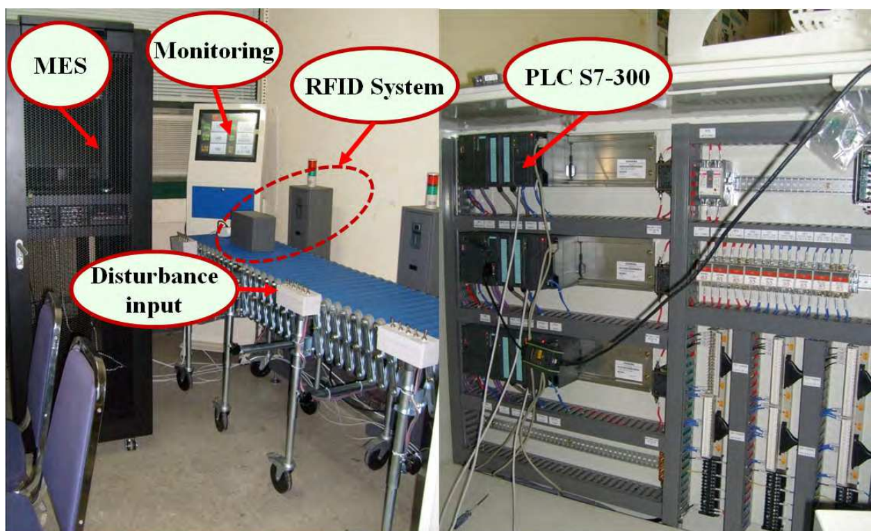
Fig. 10. Experimental setup
