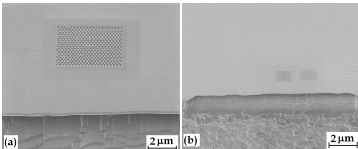
Fig. 16. a) Tilted view of the L3 cavity taken with FIB at different tilt and magnification. b) larger image of the membrane and the cavities
