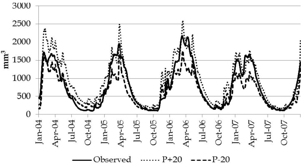
Fig. 4. Observed and Simulated runoff for scenarios P+20 and P-20
