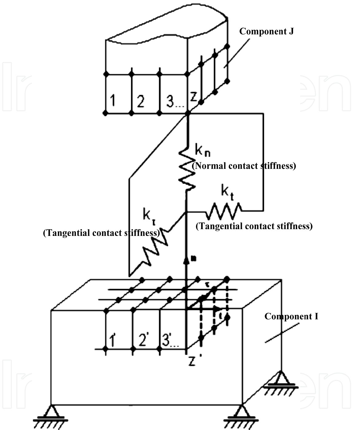
Fig. 3. Contact Model of Two Fixture Components
