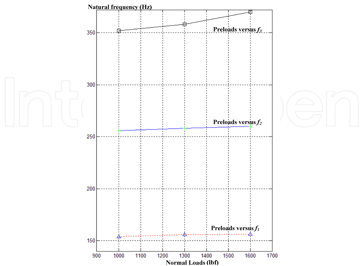
Fig. 11. The relationships between the natural frequencies and preloads
