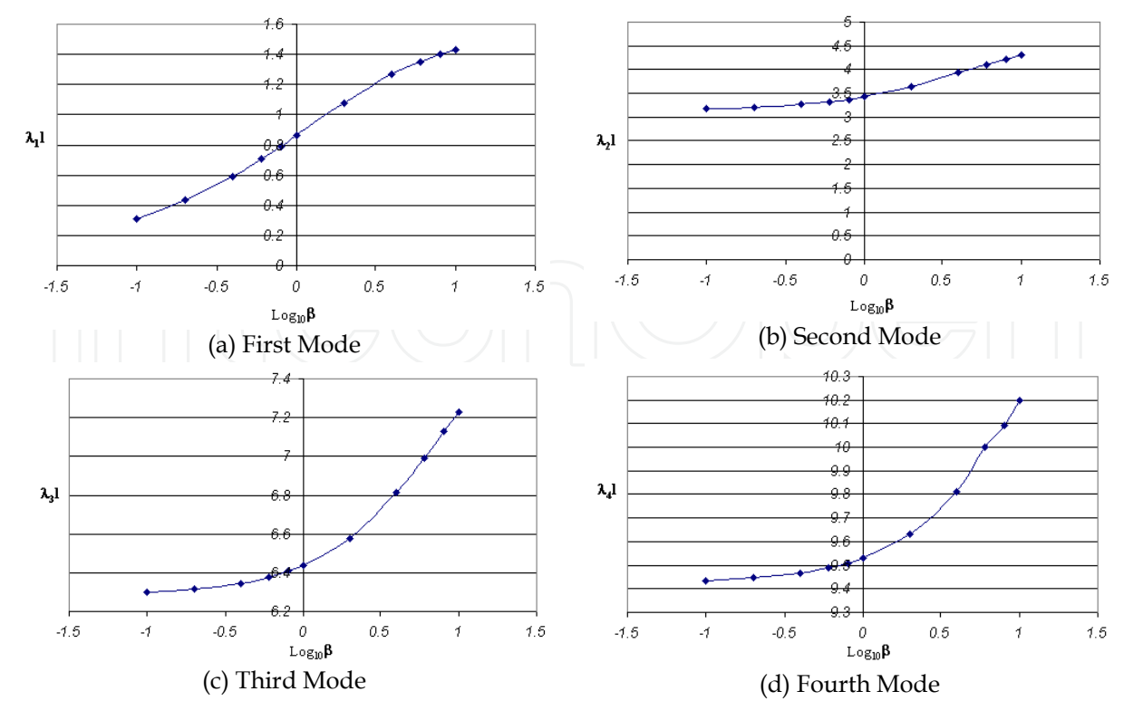
Fig. 8. Relationships between the Nondimensional Natural Frequencies and the Stiffness Ratio \beta in the First Four Modes
