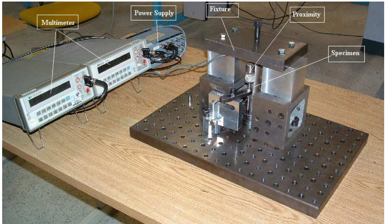
Fig. 9. Measurement Setup
