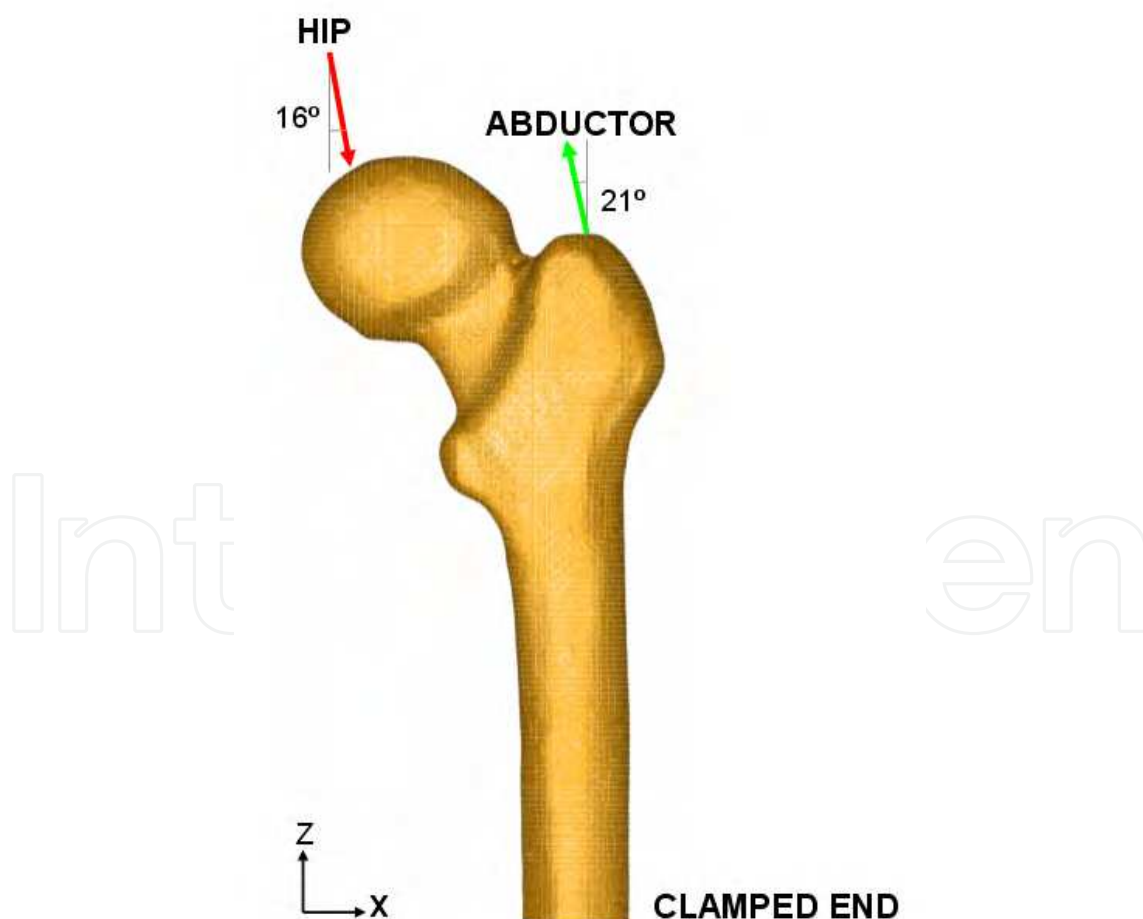
Fig. 12. Boundary conditions applied in the healthy femur model. Similar conditions are used in the implanted models
