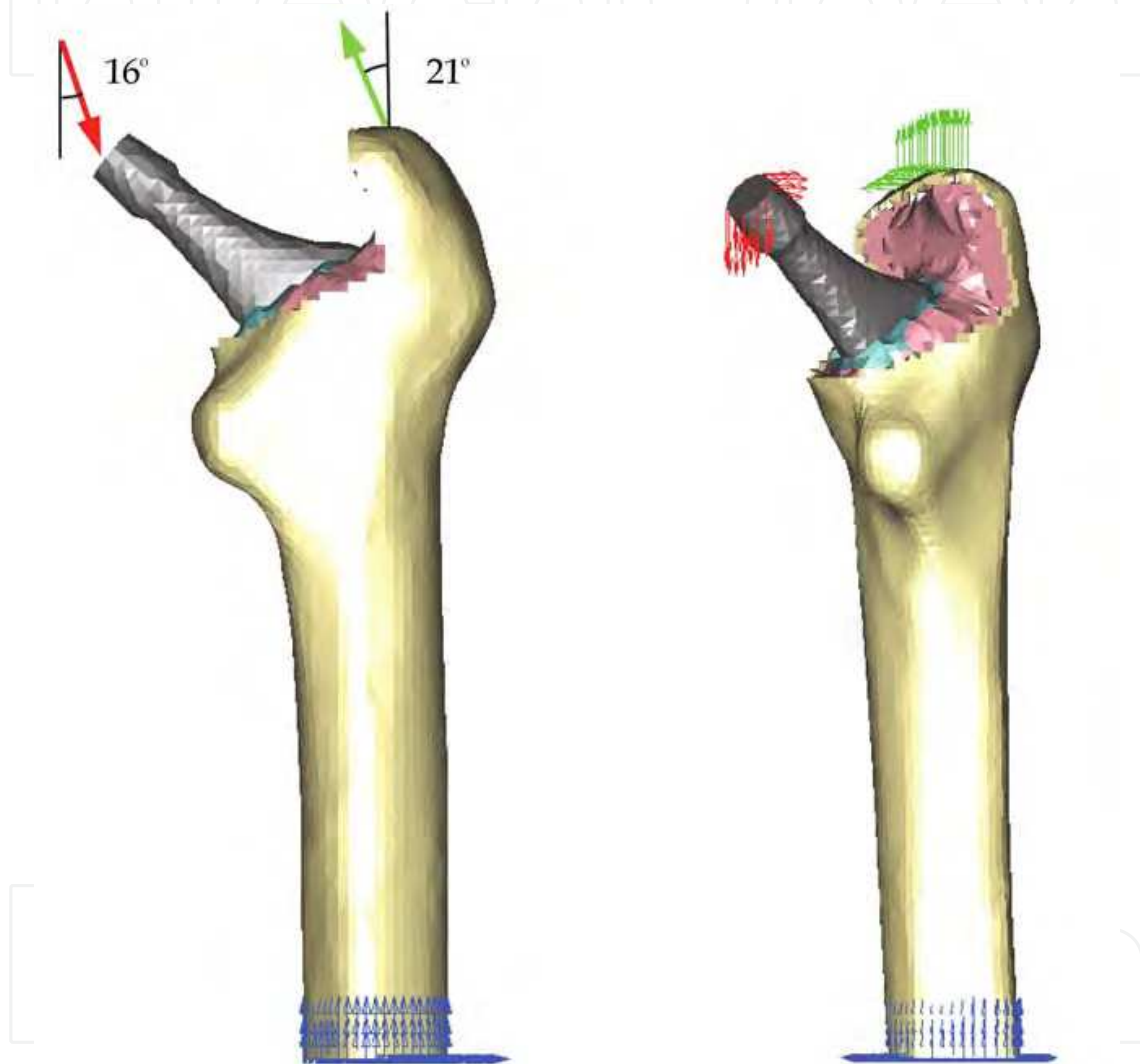
Fig. 20. Boundary conditions
