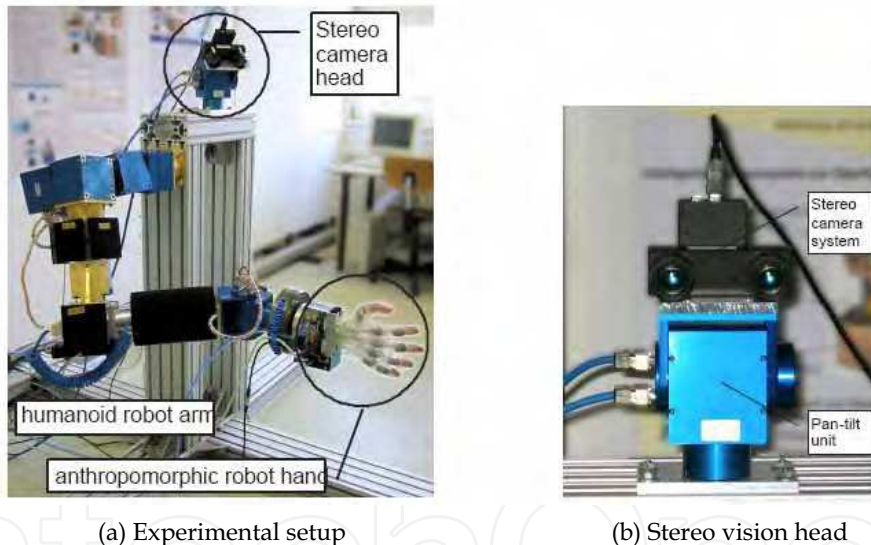
Figure 3. Robotic system framework. (a) An humanoid robot arm (7DOF) and an anthropomorphic robot hand (10DOF). (b) Stereo vision system
