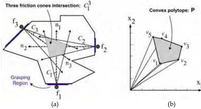
Figure 2. Feasible solution of a three-fingered grasp
