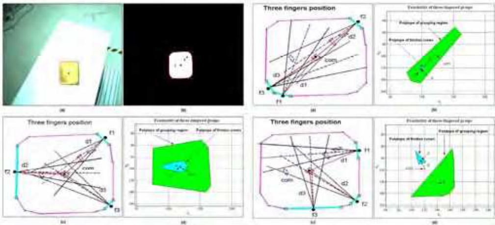
(a) Grasp configuration (GC): 1 (b) Grasp configuration (GC): 2-3 Figure 9. (a) Grasp planning setup. (b) Result of three fingered grasp configuration 1 to 3 for object obj1
