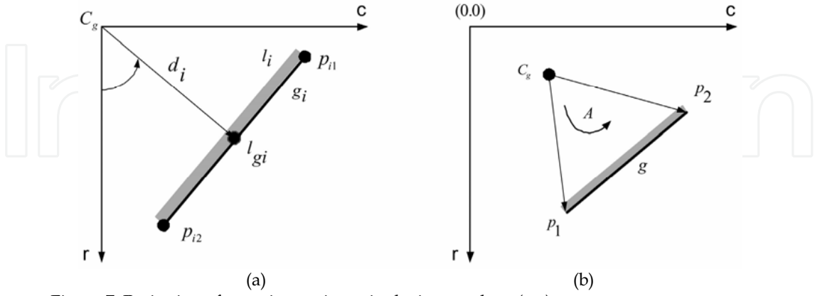
Figure 7. Projection of grasping region g_i in the image plane (c, r)
