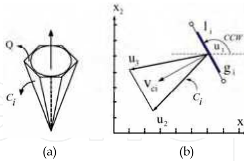
Figure 1. Point Contact Modelling
