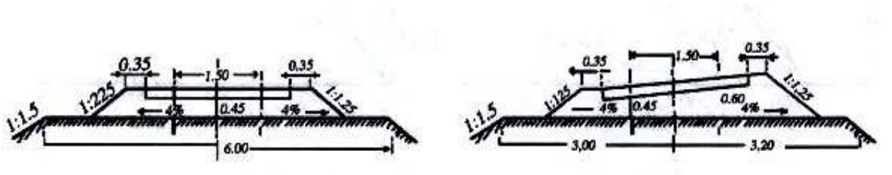
Fig. 4. Section of the different types of ballasted railway tracks in German (dimensions are in meters)
