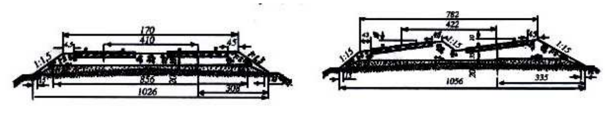
Fig. 5. Sections of railway track in the former Soviet Union (the dimensions are in cm)
