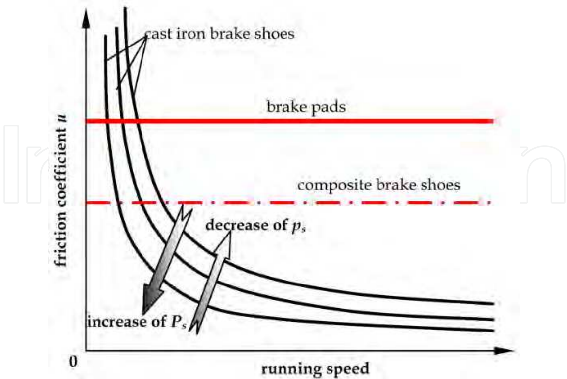
Fig. 11. Dependence of friction coefficient on running speed for different braking systems.
