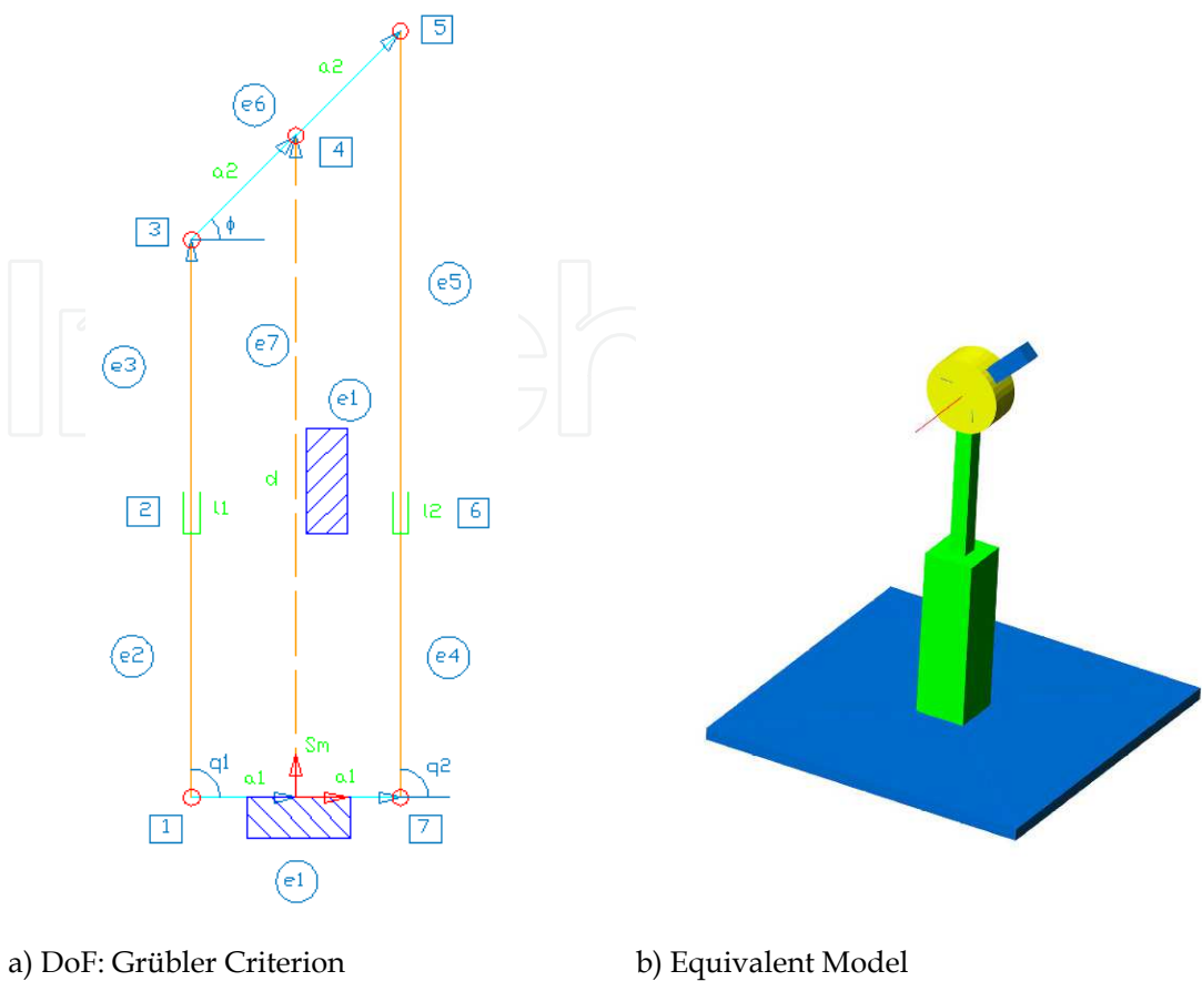
Fig. 8. Closed-chain module
