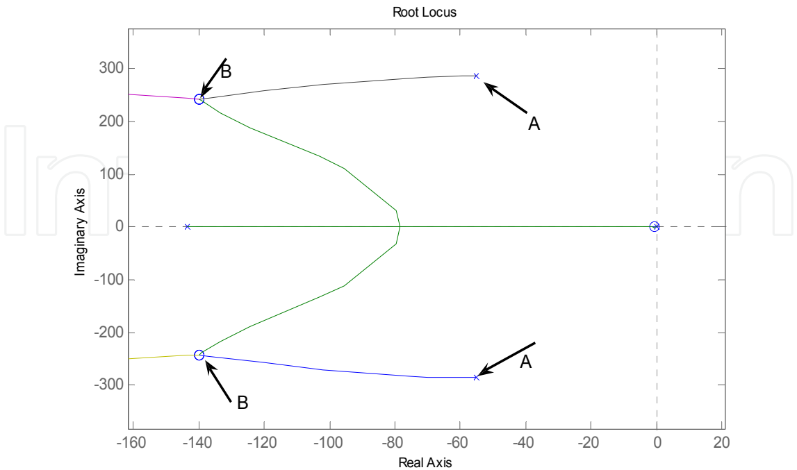
b) Poles and Zeros cancellation of the notch filter
