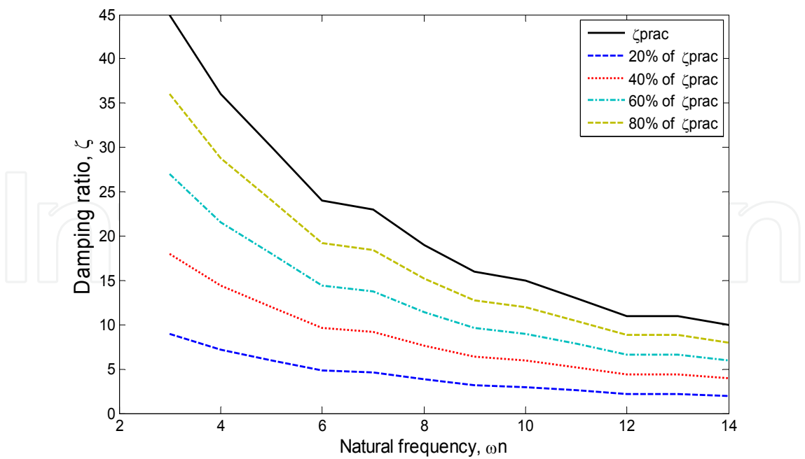
Fig. 7. Practical stability limit respecting a various margin of safety
