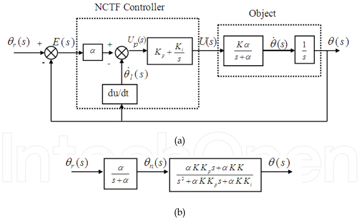
Fig. 6. NCTF control system near the origin: (a) Linearized block diagram, (b) Linearized closed-loop transfer function
