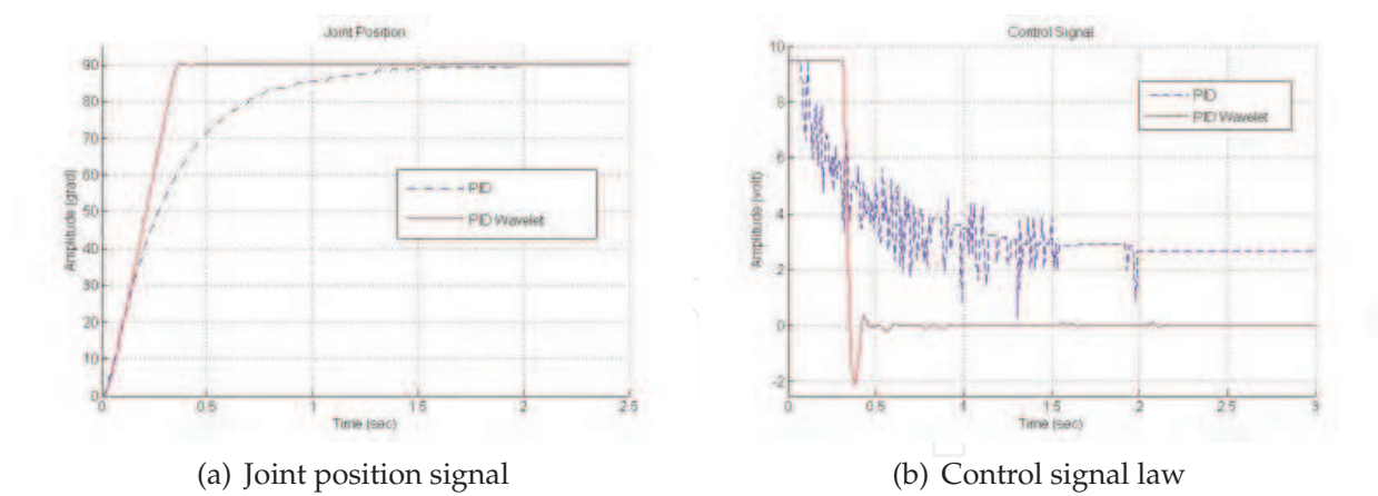
Fig. 9. Result of the joint position and control signal on the system with PID and MRPID controllers
