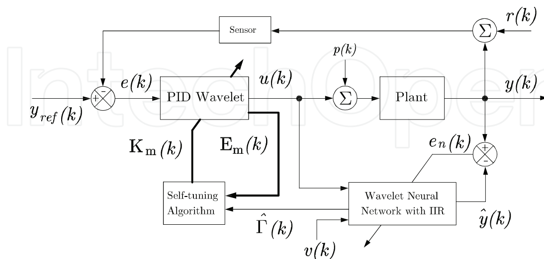
Fig. 23. Close loop block diagram of a SISO system with wavenet PID
