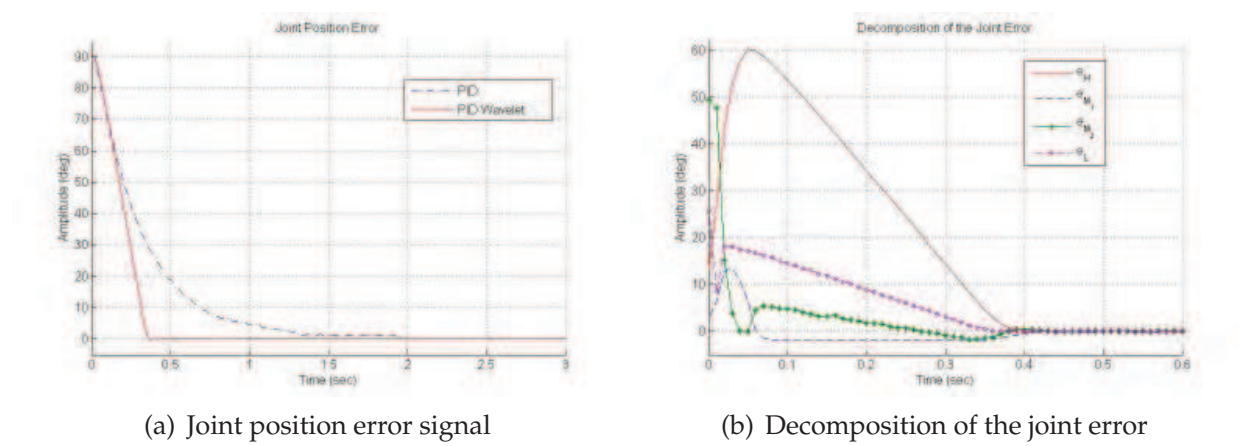
Fig. 10. Results and decomposition of the error signal on the system with PID and MRPID controllers
