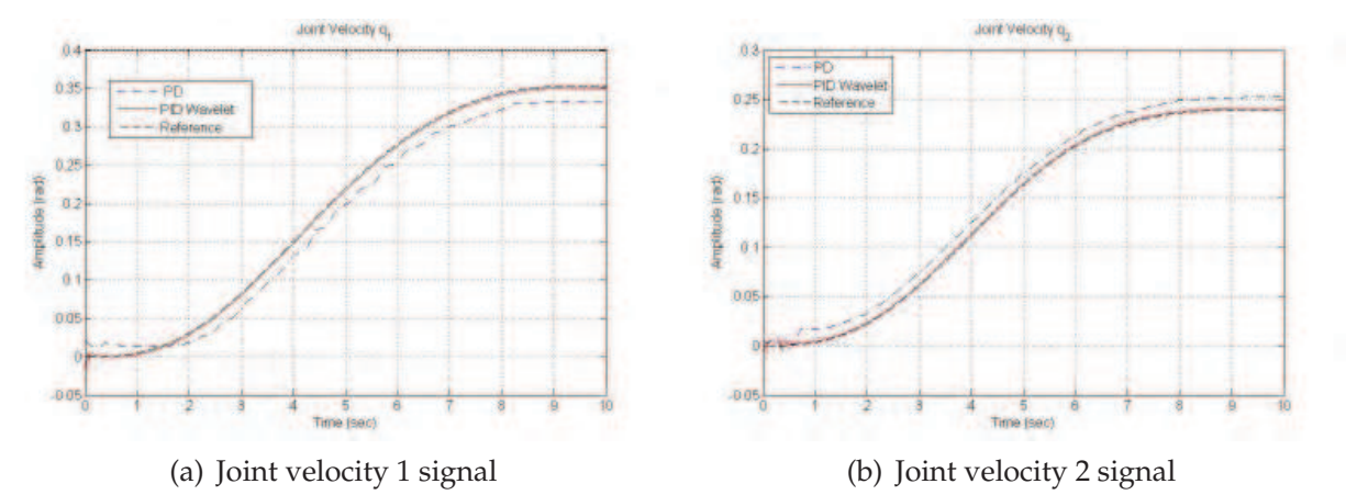
Fig. 18. Results of the speed signal to the actuator joint 1 y 2
