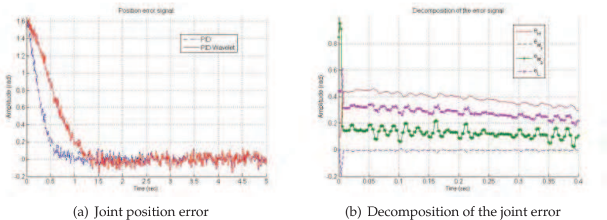
Fig. 7. Results and decomposition of the error signal on the system with PID and MRPID even in the presence noise
