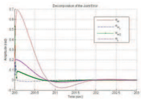
Fig. 25. Decomposition of the error signal
