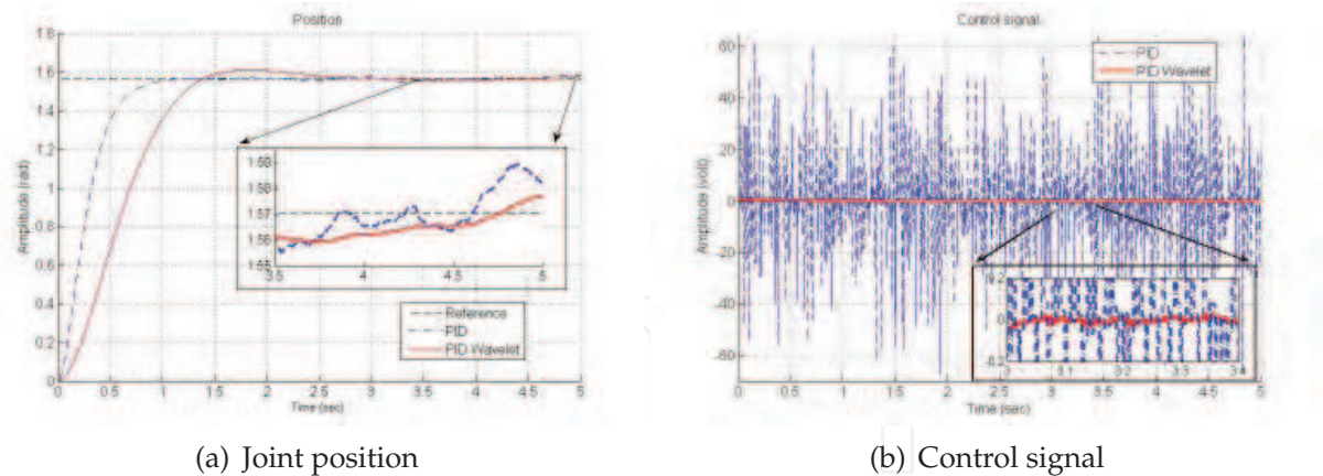
Fig. 6. Results of the position and control signal on the system with PID and MRPID controller even in the presence of noise
