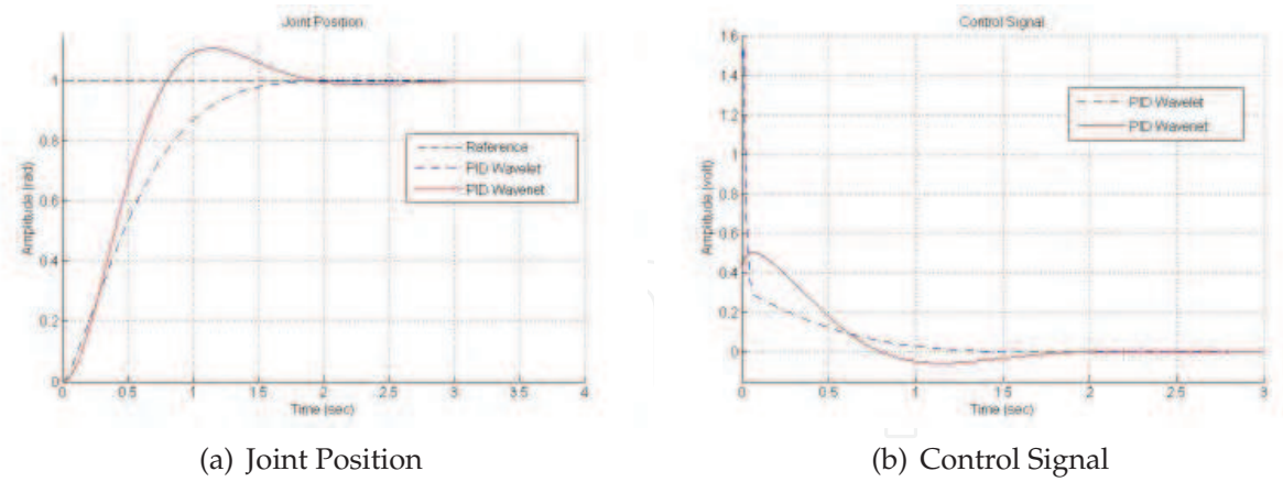
Fig. 24. Result of the joint position and control signal on the system with MRPID and wavenet PID controller
