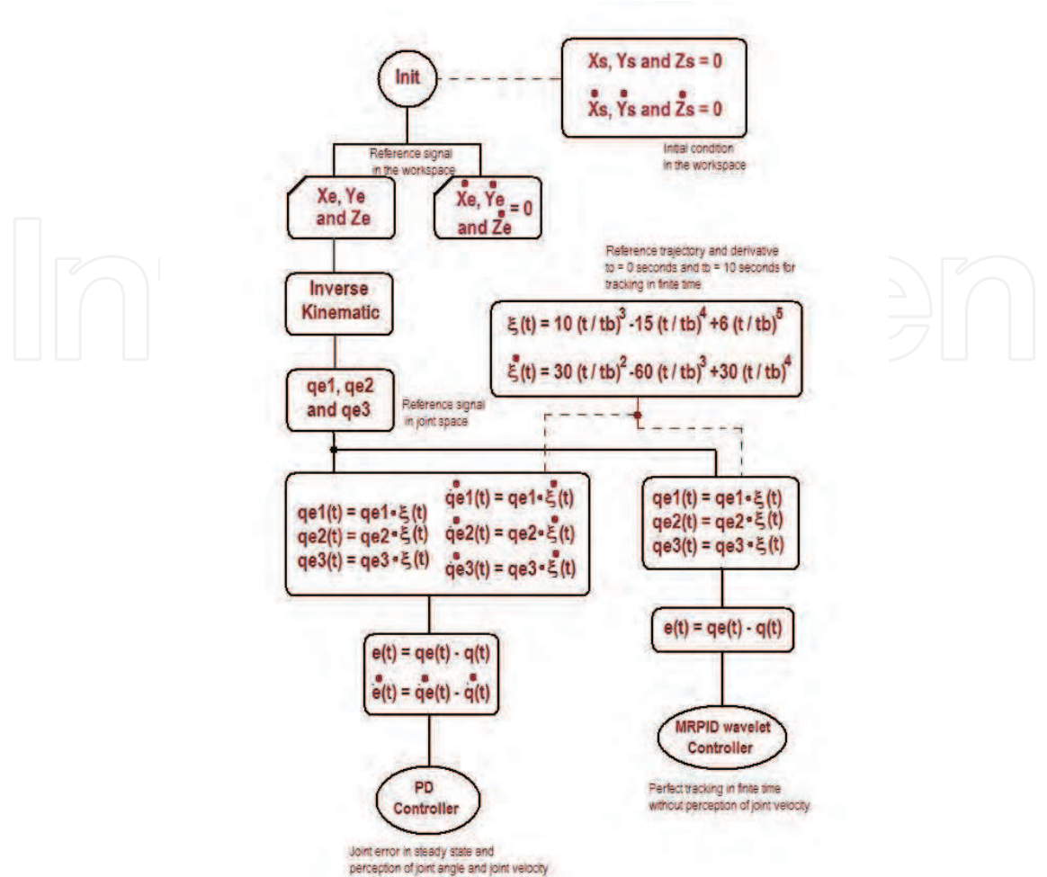
Fig. 15. Block diagram which illustrates the flow of information between the two controllers employed.
