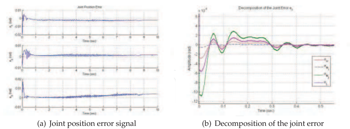
Fig. 17. Results and decomposition of the error signal on the system with MRPID
