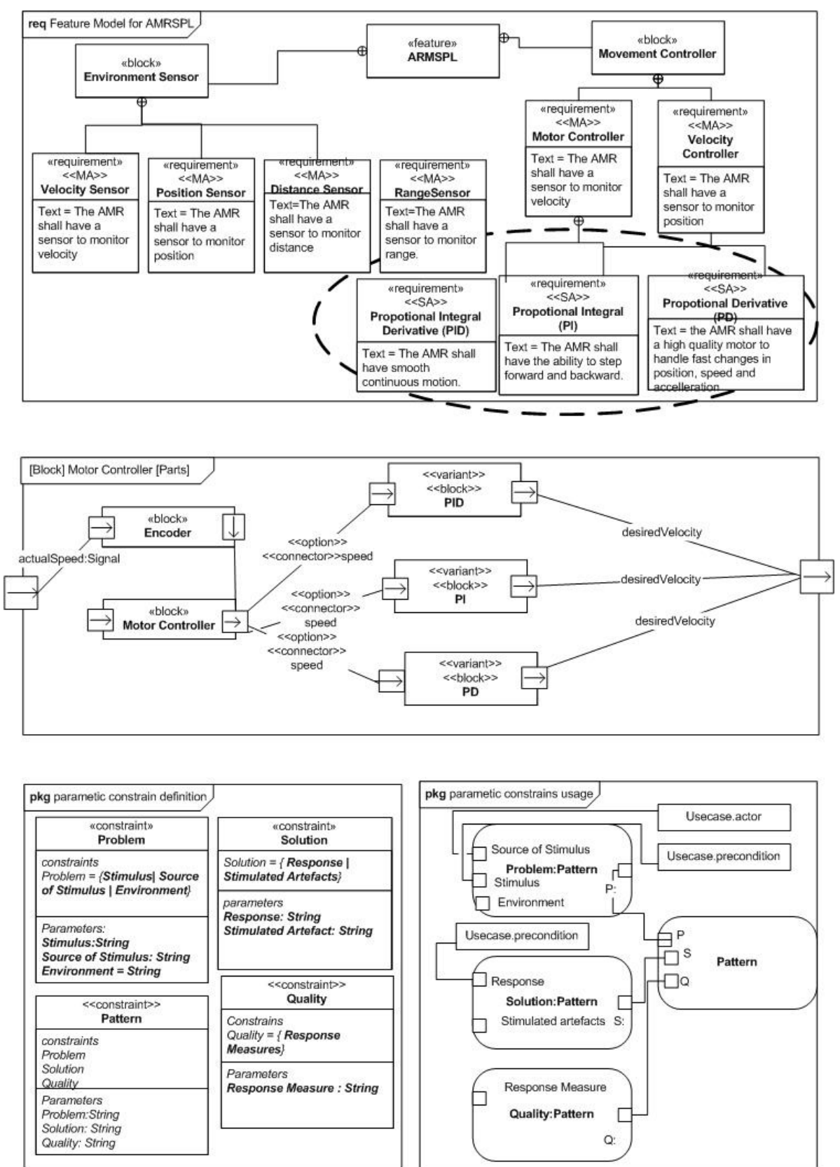
Fig. 9. Vertical mapping between Feature Model, Parametric Model and Component Connector Model of AMRPL
