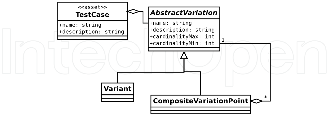
Fig. 8. The metamodel for tests.
