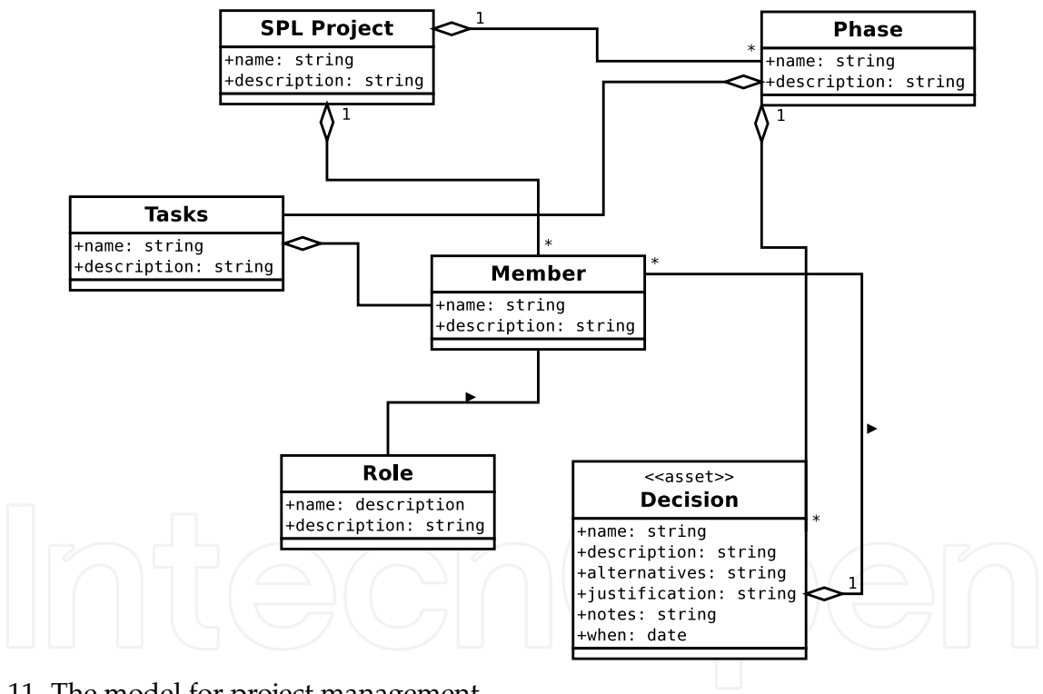
Fig. 11. The model for project management.
