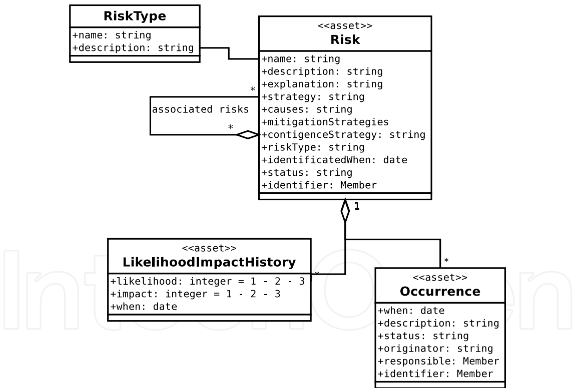
Fig. 12. The metamodel for risks management.
