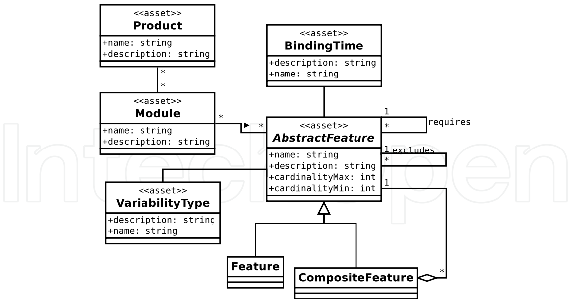
Fig. 6. The model for scoping phase.
