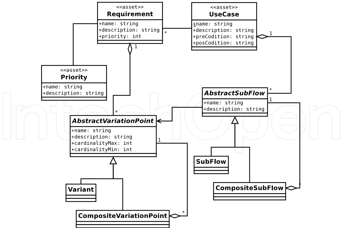
Fig. 7. The metamodel for requirements phase.
