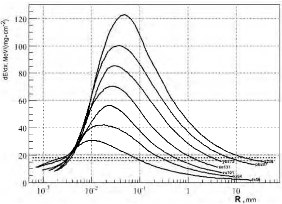
Fig. 19. Ionization losses of _{26}^{56}\text{Fe} , _{36}^{84}\text{Kr} , _{44}^{101}\text{Ru} , _{54}^{131}\text{Xe} , _{70}^{173}\text{Yb} , _{82}^{207}\text{Pb} , _{92}^{238}\text{U} nuclei in olivine depending on the residual run.
