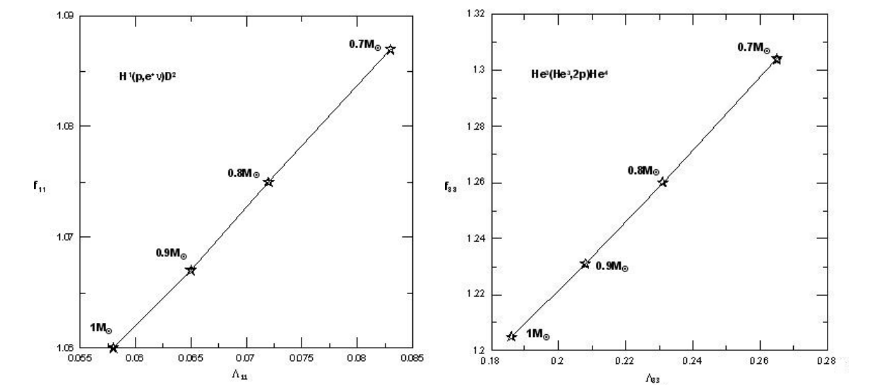
Fig. 1. Variation of the screening factors (S54) for H^1(p,e^+\nu)D^2 reaction with the screening strength parameter \Lambda (left). Variation of the screening factors (S54) for He^3(He^3,2p)He^4 reaction with the screening strength parameter (right)
