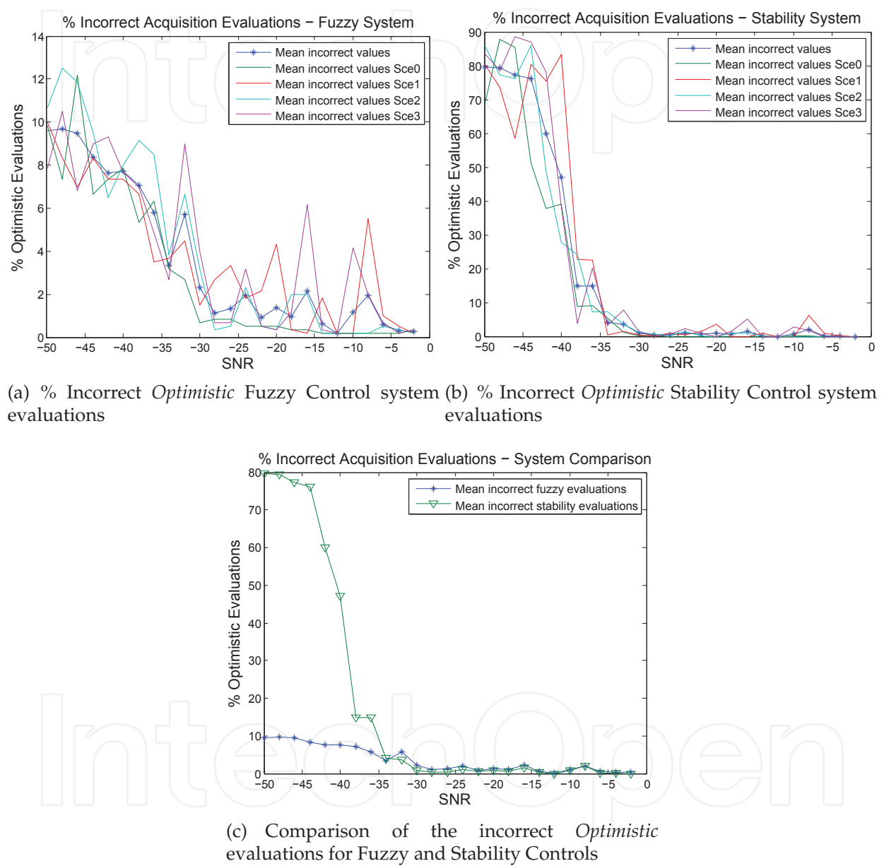
Fig. 18. Comparison of the incorrect evaluations for both fuzzy and stability controls, in case that the error is optimistic .
