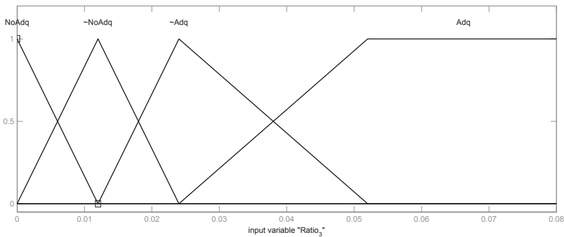
Fig. 11. Membership functions for input variable Ratio_3
