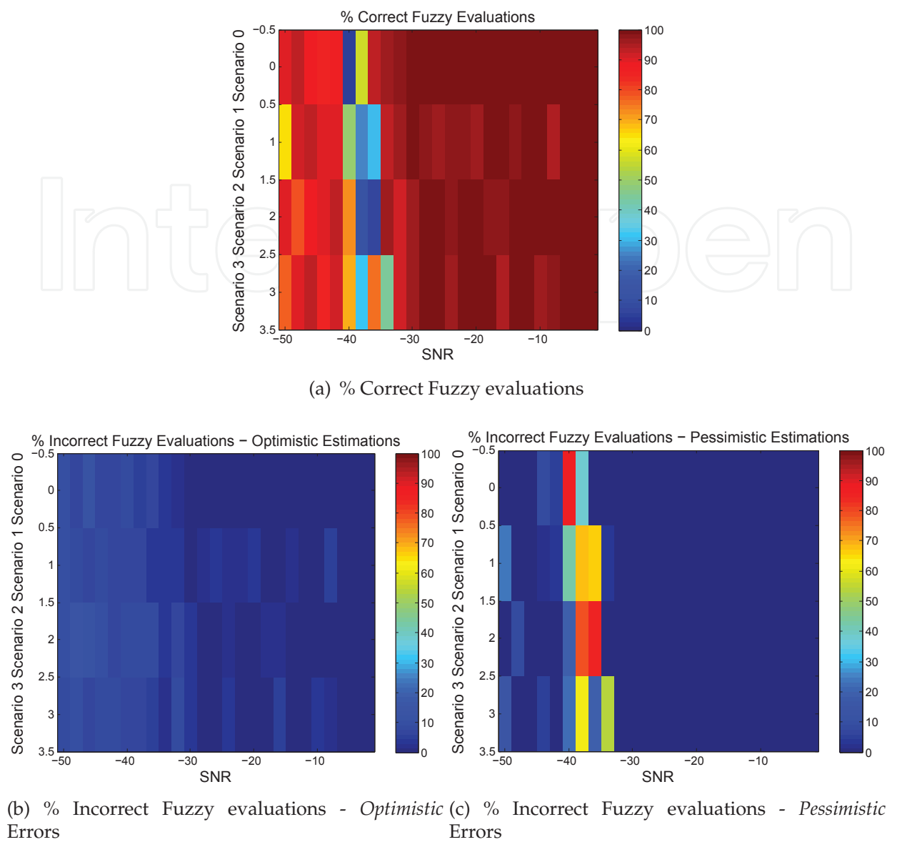
Fig. 15. Performance of the Fuzzy Logic Control. Measurements about the correct and incorrect evaluations. factor, it must be taken into account that some bad estimations ( pessimistic ones) prevent the system from obtaining better information ratios in certain ranges of SNR [-38,-35] dB.
