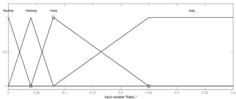
Fig. 9. Membership functions for input variable Ratio_1
