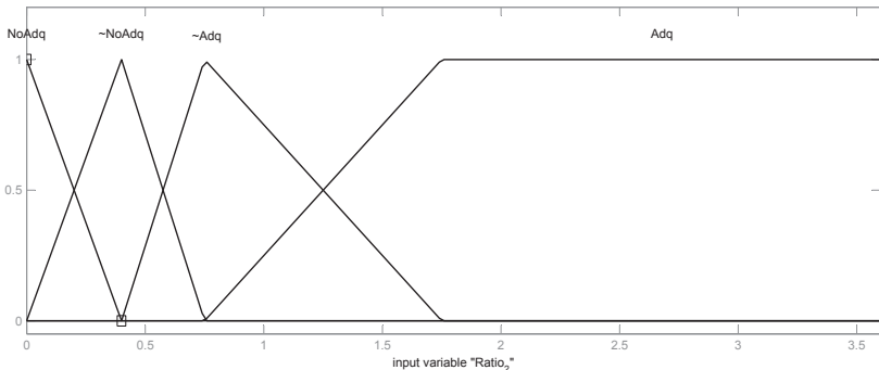
Fig. 10. Membership functions for input variable Ratio_2
