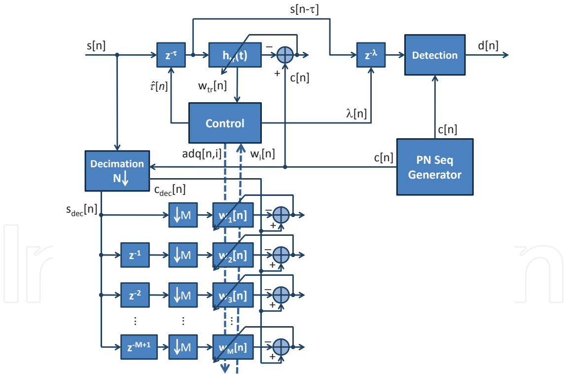
Fig. 2. Multiresolutive structure for acquisition and tracking
