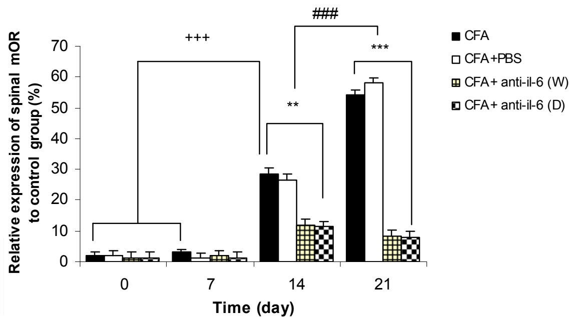
Fig. 4. CFA injection caused significant increased in spinal mOR expression time dependently. Anti- IL-6 antibody administration significantly reduced spinal mOR expression during different stages of AA. Ratio of spinal mOR protein band intensity in AA group significantly decreased at 14 th and 21 th days after anti-IL-6 antibody treatment compared to AA control group. Data are presented as mean \pm SEM (n=6/ group). +++ P < 0.001 comparison of ratio of spinal mOR protein band intensity between different days of AA. ** P < 0.01 , *** P < 0.001 comparison of spinal mOR protein band intensity between AA and AA + anti-IL-6 antibody treated rats. ### P < 0.001 indicated spinal mOR protein band intensity difference in AA and AA + anti-IL-6 antibody treated rats between 14 th and 21 th days.
