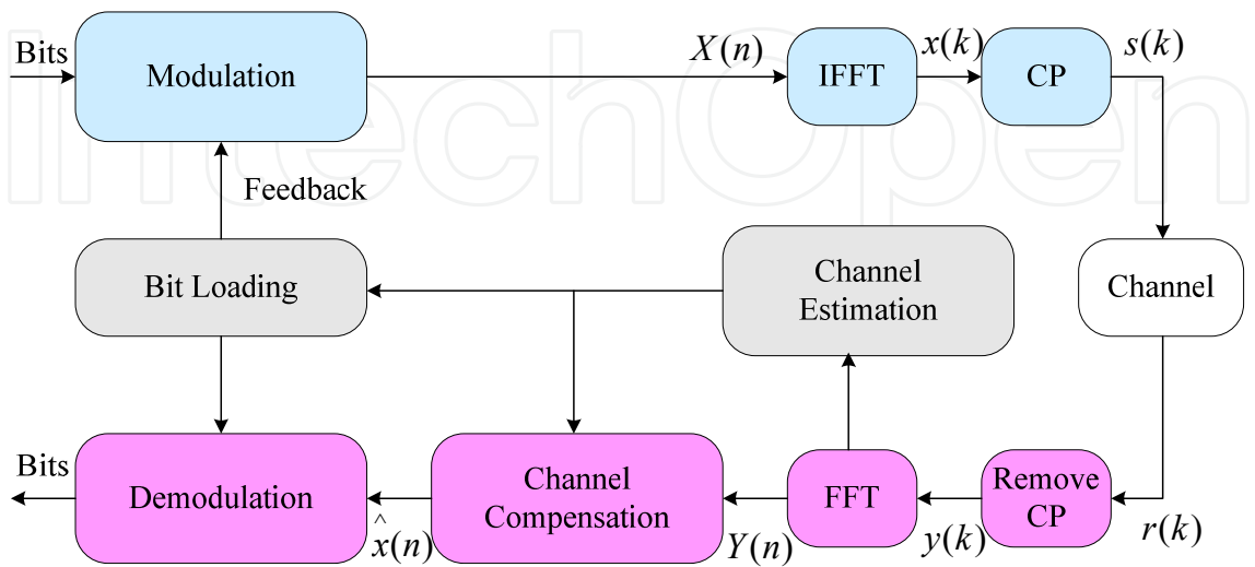
Fig. 2. OFDM system
