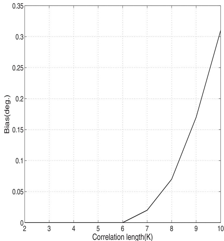
Fig. 12. Bias of the estimated direction according to spatial correlation length of the noise.
