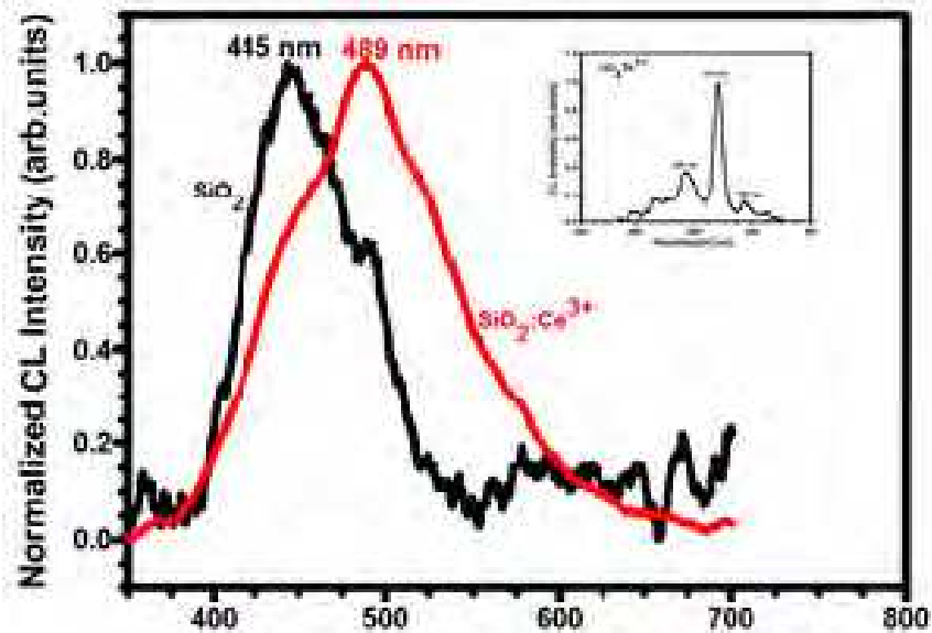
Fig. 5. Normalized CL intensity of SiO 2 and SiO 2 :Ce 3+ . The inset is the CL intensity versus wavelength spectrum of SiO 2 :Tb 3+ .
