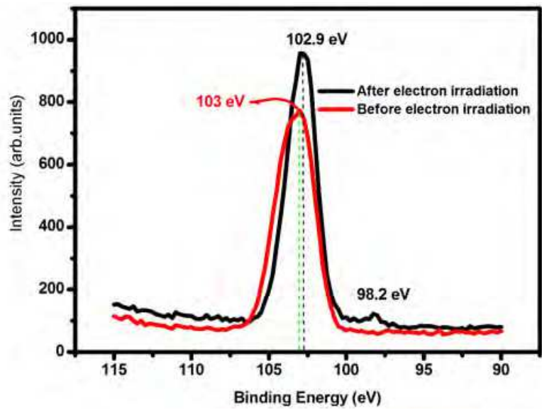
Fig. 11. High resolution Si XPS peaks before and after electron irradiation.
