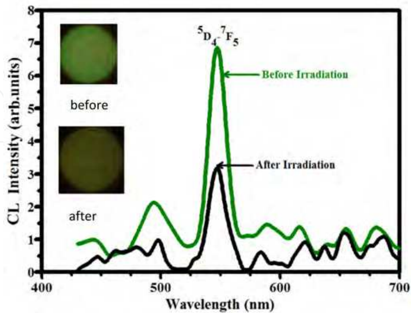
Fig. 6. CL intensity spectra of SiO 2 :Ce 3+ ,Tb 3+ before and after electron irradiation.
