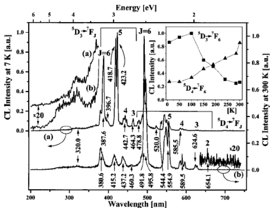
Fig. 3.6. CL spectra of a-AlN:Tb recorded at cryogenic and room temperature. The inserts show the total integral intensity of the dominant 4f-shell transition lines as a function of temperature. After Ref. [(Jadwisieniczak, Lozykowski et al. 2000)].
