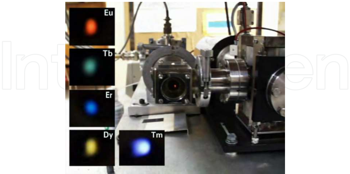
Fig. 2.5. Front view of a low temperature cathodoluminescence experimental setup operating between 6K- 330K and electron acceleration voltage up to 20 kV. Insets show color emissions from different RE-doped III-nitrides.
