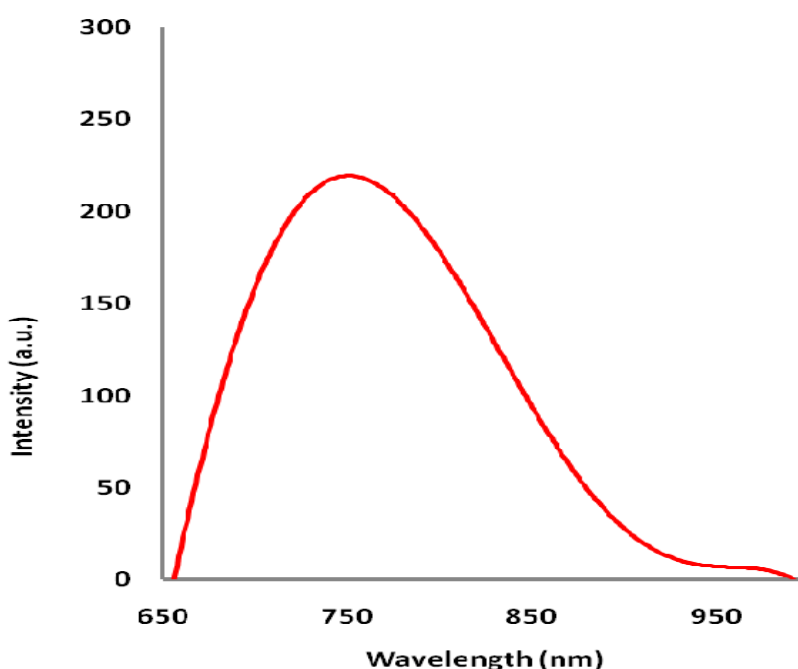
Fig. 4.8. Cathodoluminescence spectrum of amorphous AlN:Ti.
