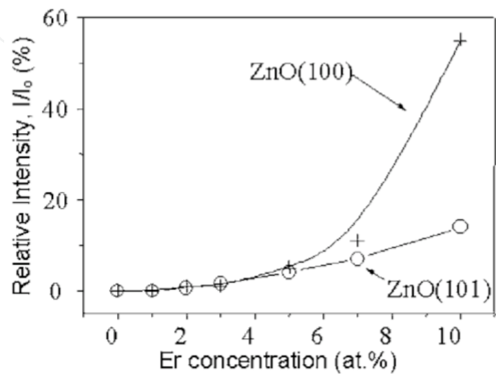
Fig. 18. Relative integrated intensity I/I_o of the 100 and 101 x-ray peaks measured from the intensity I_o of the 002 peak with respect to Er content in the investigated samples.
