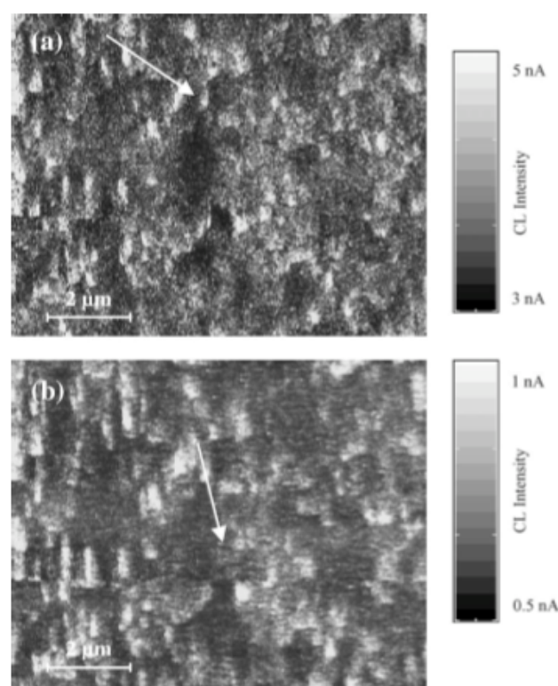
Fig. 15. Cathodoluminescence image of F-doped ZnO thin film taken at 4 keV: (a) polychromatic CL image, (b) monochromatic CL image taken at \lambda=372\pm8 nm. The full arrow in each image is a marker for the investigated region of the film surface area.
