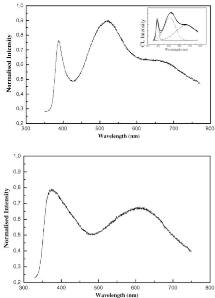
Fig. 12. Cathodoluminescence spectra of: (a) undoped ZnO and (b) Sn-doped ZnO films at E=5 keV electron beam energy with a beam current of about 1 nA.
