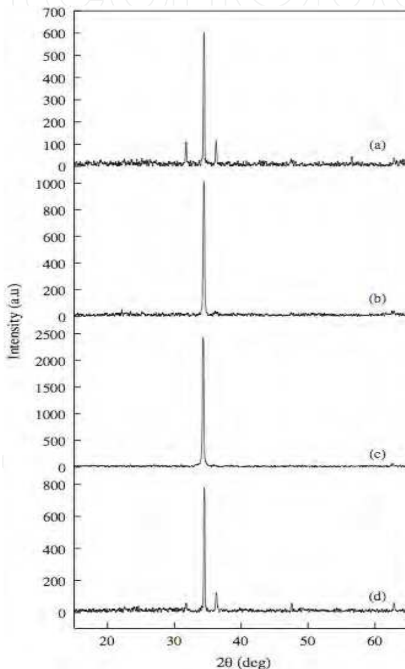
Fig. 3. XRD of ZnO sprayed at flow rate f=5\text{ml/min} deposited on different temperature: (a) : T=350^\circ\text{C} , (b): T=400^\circ\text{C} , (c) : T=450^\circ\text{C} , and (d) : T=500^\circ\text{C} .
