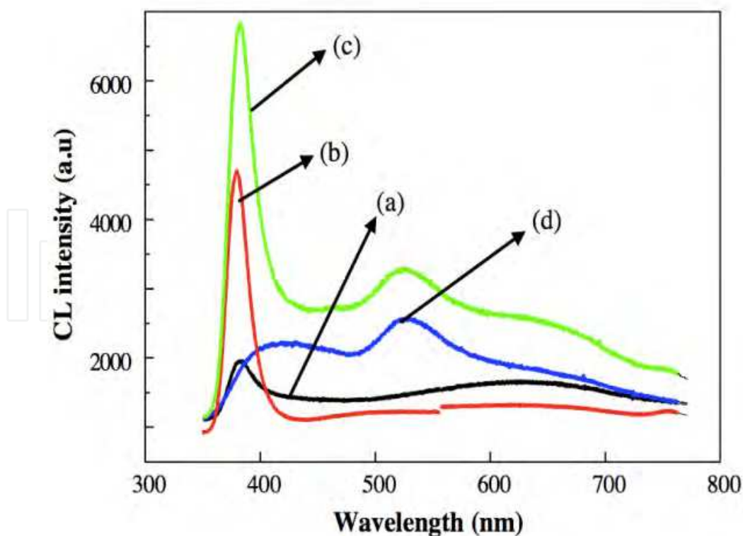
Fig. 2. CL Spectra of ZnO sprayed at flow rate f=5 ml/min deposited on different temperature: (a) : T=350^{\circ}\text{C} , (b): T=400^{\circ}\text{C} , (c) : T=450^{\circ}\text{C} , and (d) : T=500^{\circ}\text{C} .
