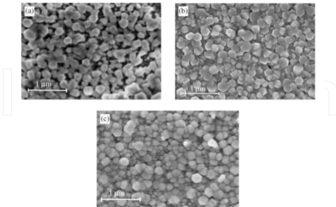
Fig. 6. SEM micrographs of ZnO films sprayed at substrate temperature T_s=450\text{ }^{\circ}\text{C} and different air flow rate: (a) f=2.5\text{ ml/min} , (b) f=5\text{ ml/min} , (c) f=7.5\text{ ml/min} and substrate temperature: T_s=450\text{ }^{\circ}\text{C} .
