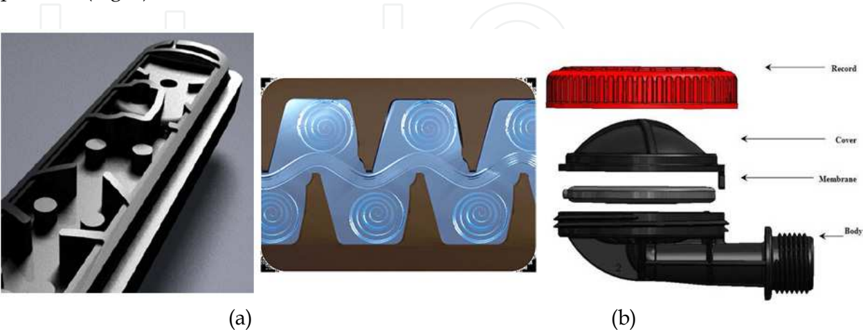
Fig. 3. Elements of SDI units: (a) emitter models and (b) flushing bulb. (Courtesy of NaaDanJain Irrigation).
