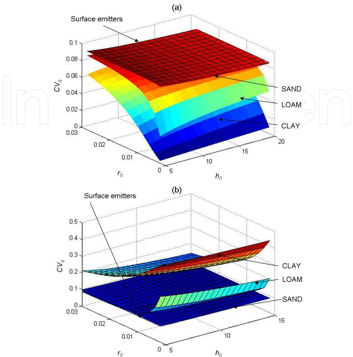
Note: Units for r_0 and h_0 are expressed in m. Fig. 12. Irrigation uniformity index CV_q as a function of r_0 and h_0 in different soils for a SDI lateral with non-compensating emitters: (a) uniform soils; (b) non-uniform soils. Uniformity of water application in all cases reduces as inlet pressure increases. Consequently, it would be advisable to select emitters with small discharge, and to irrigate with inlet pressure not very small (in this case above 10 m).
