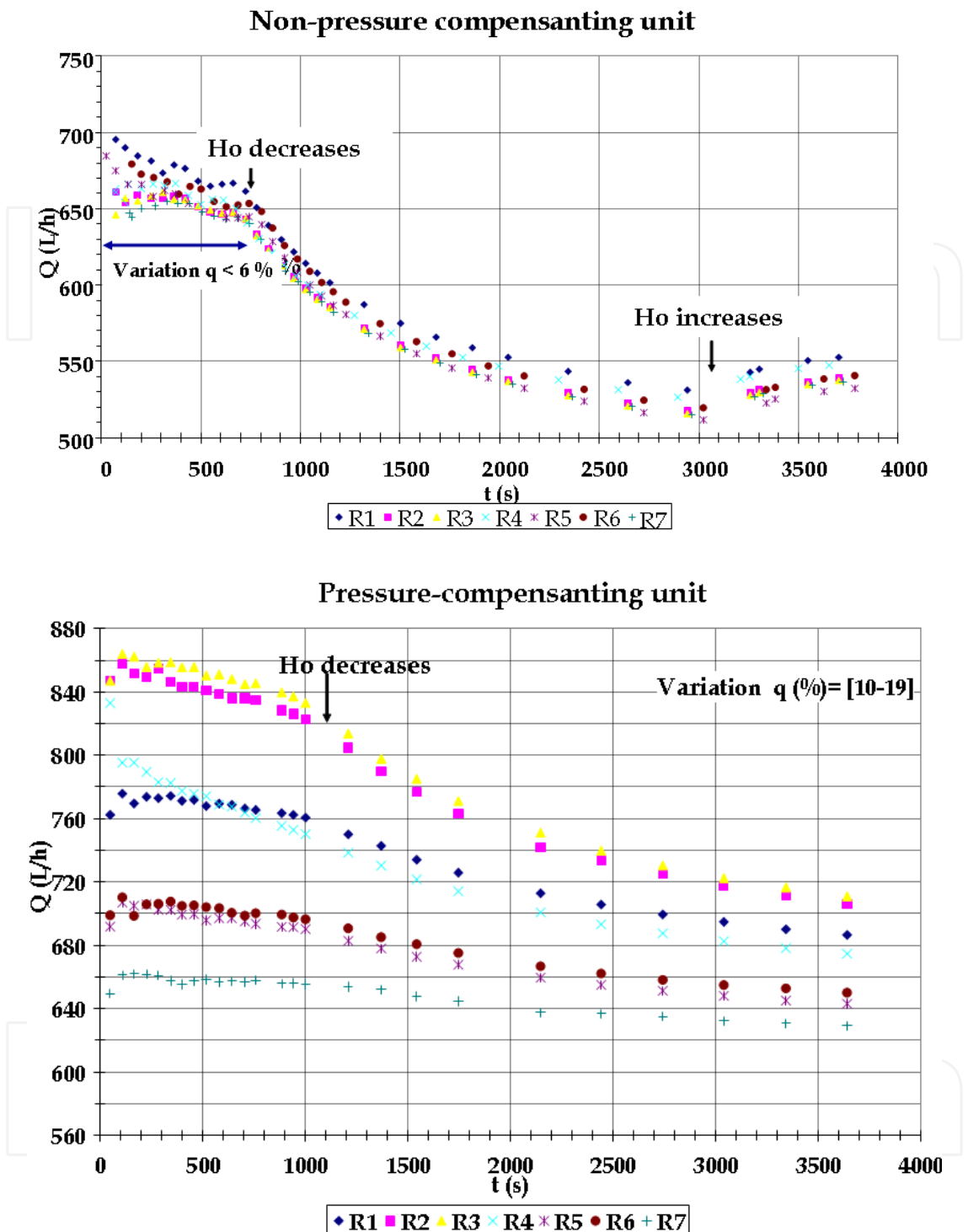
Fig. 9. Variation of lateral inlet flow of a SDI unit laid on a loamy soil during irrigation (Note: Ri= lateral).
