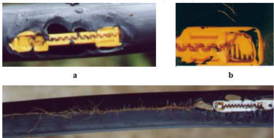
Fig. 11. Root intrusion in different emitters . (Source: Ronaldo Souza 2003)
