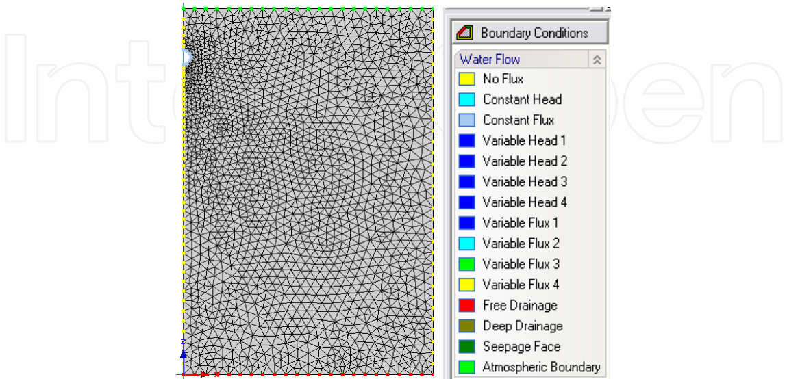
Fig. 14. Geometry, mesh and boundary conditions.
