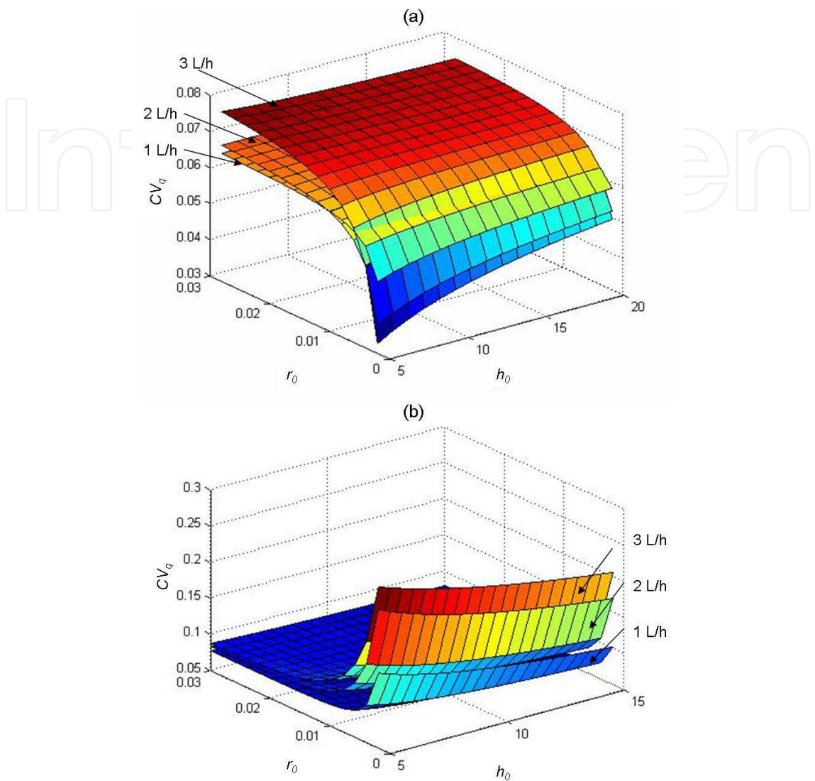
Fig. 13. Irrigation uniformity coefficient CV_q as a function of r_0 and h_0 in a SDI lateral with non-compensating emitters of different discharges: (a) loamy uniform soil; (b) loamy non-uniform soil.
