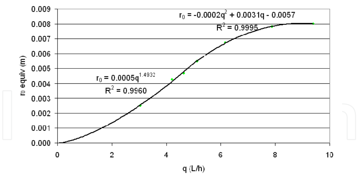
Fig. 7. Variation of the radius spherical cavity with emitter discharge in uniform soils. (Source: Gil et al. 2011).
