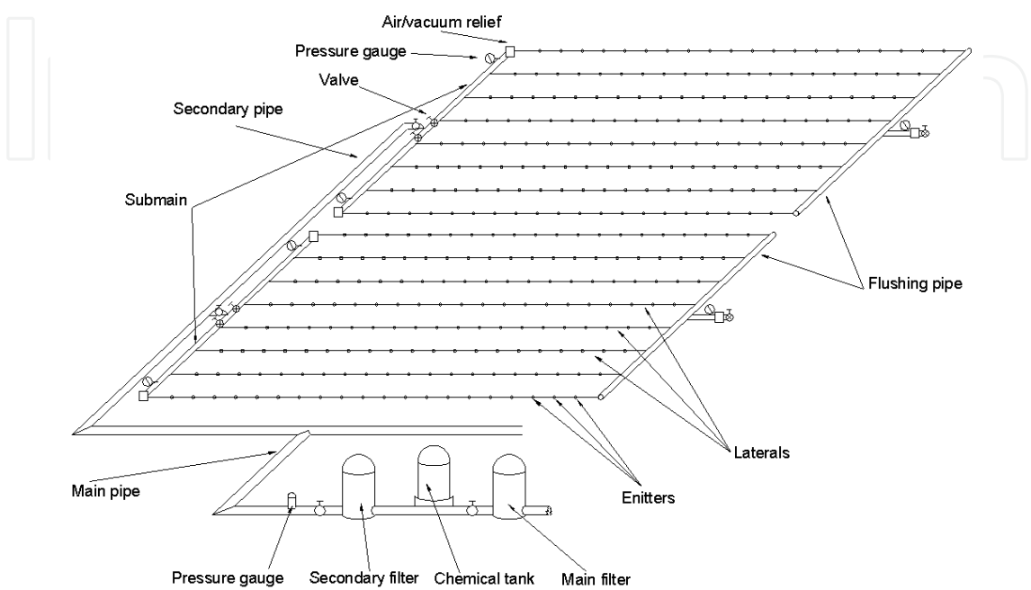
Fig. 2. Scheme of a typical SDI unit.
