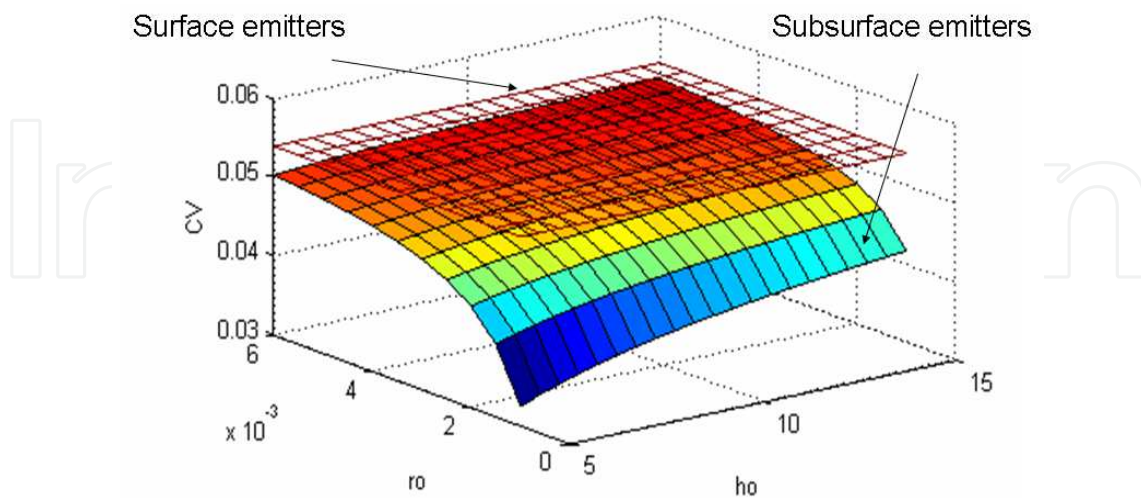
Fig. 8. Coefficient of variation of flow CV_q in laterals with 100 non regulated emitters of 2 L/h laid on a uniform loamy soil, considering hydraulic variation negligible (Note: r_0 , h_0 and h_s are expressed in m). (Source: Gil et al. 2008).
