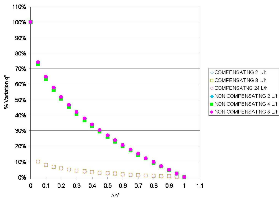
Fig. 16. Variation of q^* ( q/h_0^x ) versus \Delta h^* [(h_0 - \bar{h}_s)/h_0] for different emitter models. (Source: Gil et al. 2011).
