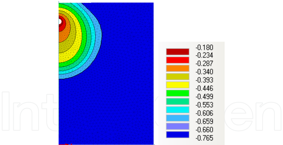
Fig. 15. Example of water distribution in a sandy soil after 4 h of irrigation ( q = 10 \text{ L/h} ).
