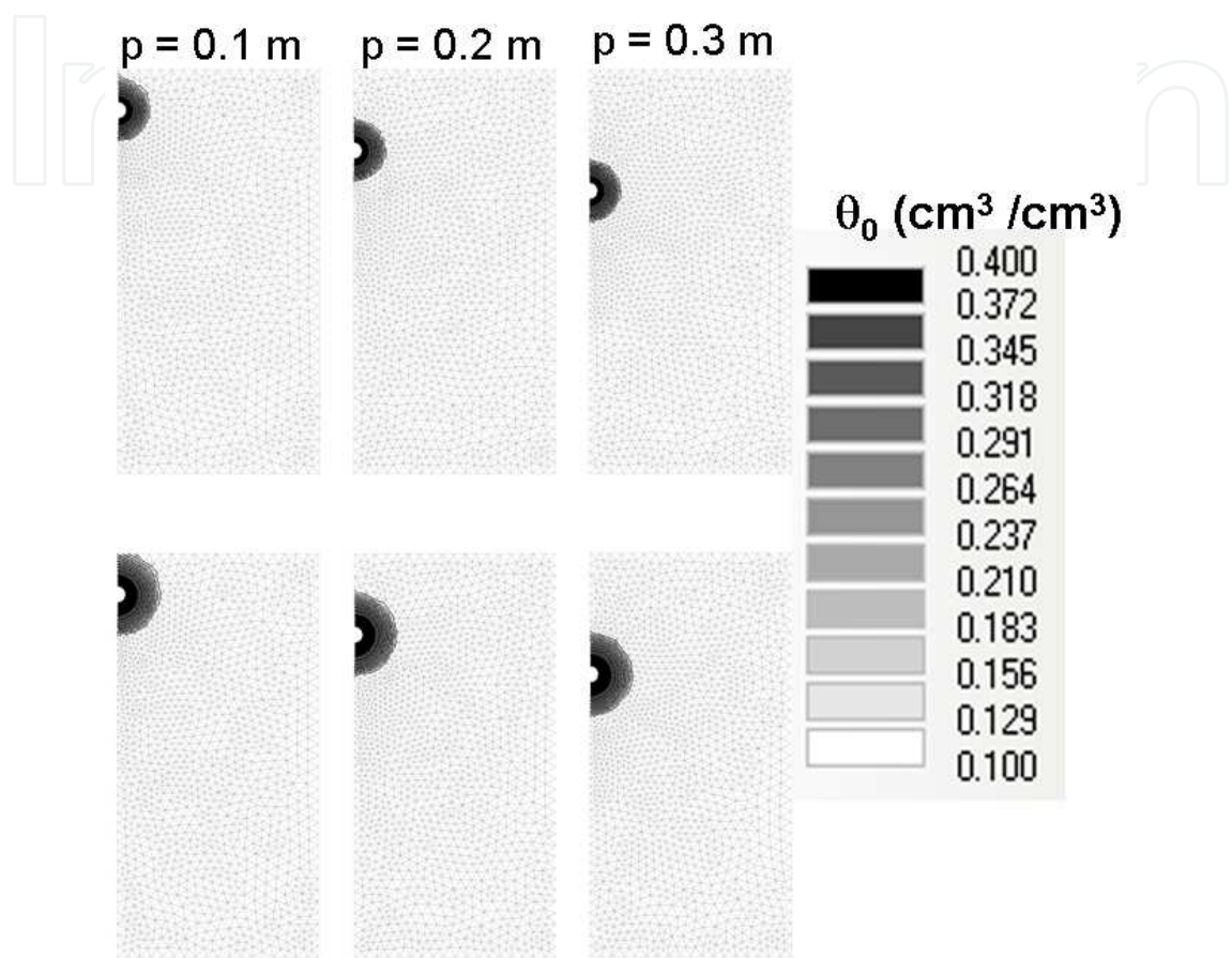
Fig. 18. Wetting bulbs of drip and a SDI in uniform loamy soil for an emitter pressure of 16 m and initial soil water content \theta_0= 0.1 .
