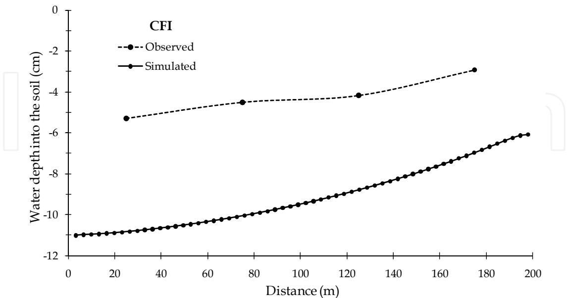
Fig. 11. Infiltration table along furrow for CFI. Observed values were monitored in 2004
