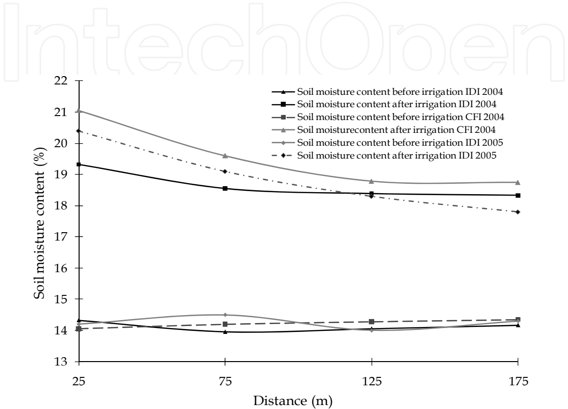
Fig. 13. Average soil moisture content before and after irrigation events (2004 & 2005)
