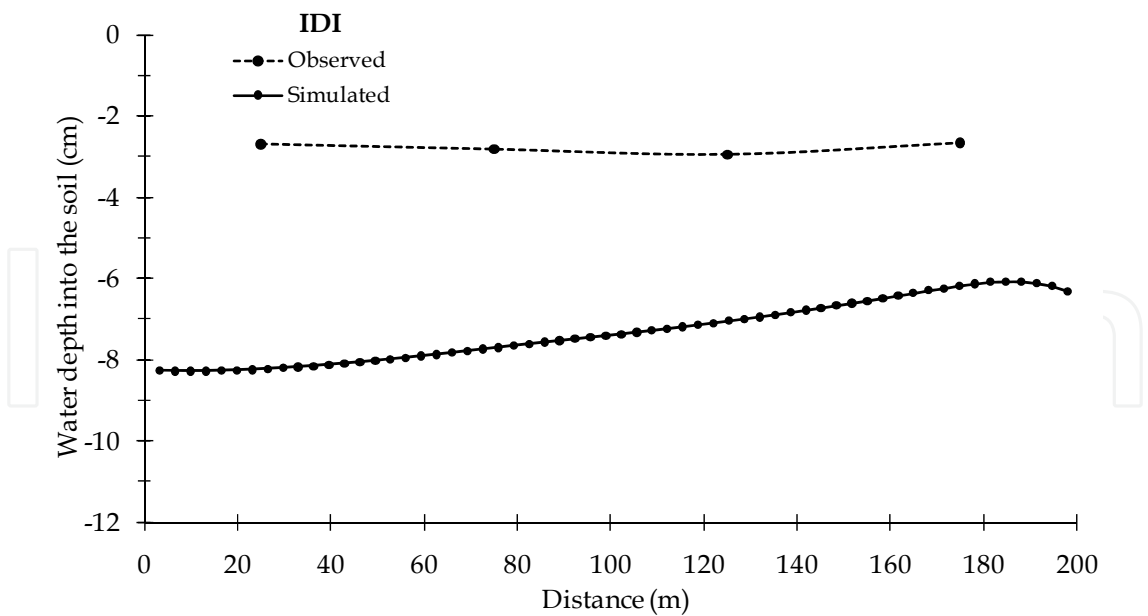
Fig. 12. Infiltration table along furrow for IDI. Observed values were monitored in 2004
