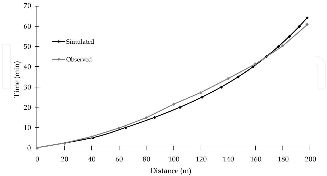
Fig. 6. Water advance curves. Pre-sowing irrigation for CFI (2004)
